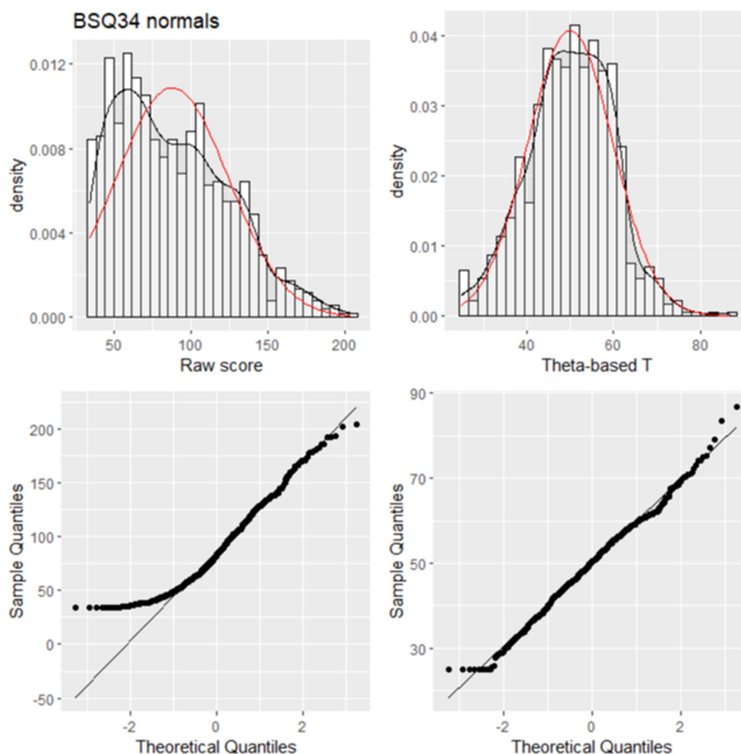
FIGURE 2 Histogram and normal probability plot for the BSQ34.
