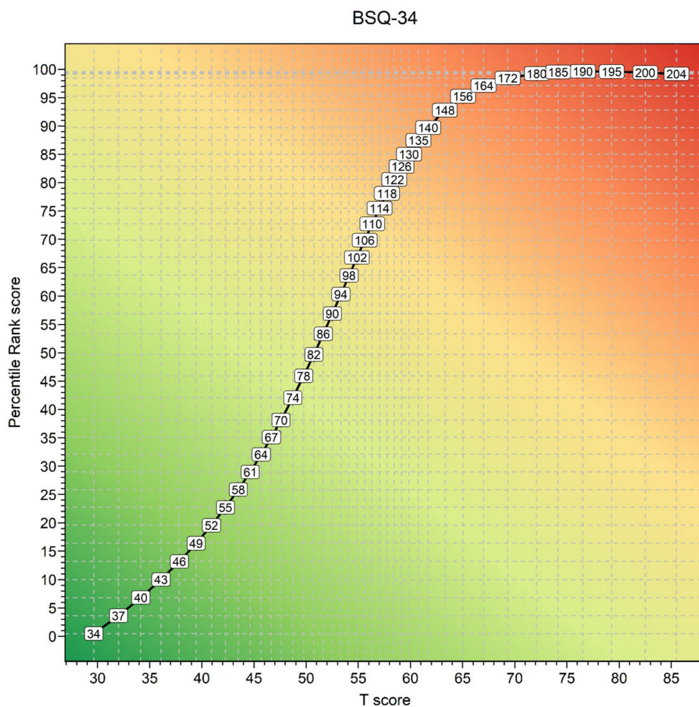
FIGURE 3 Raw scores, T -scores, and Percentile Rank scores of the Saudi-Arabic BSQ34.
