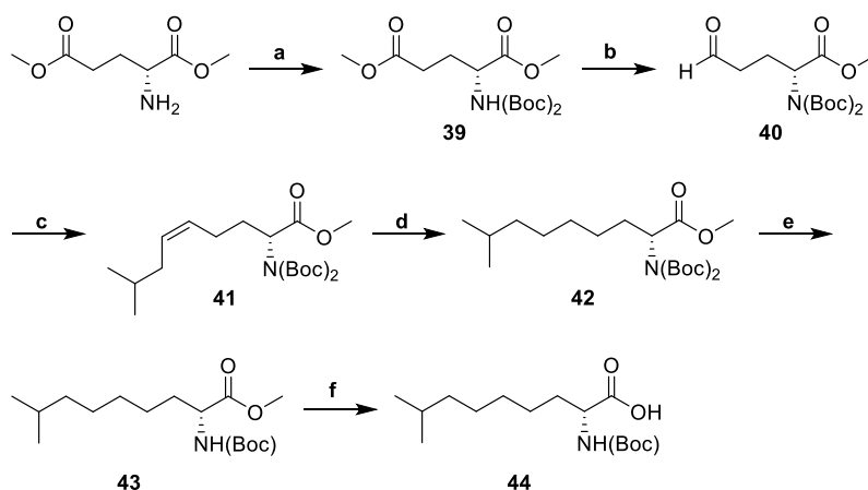
Scheme 5. Synthesis of the Polymyxin Analogue 45 Lacking a Reductively Labile Disulfide Bond a
