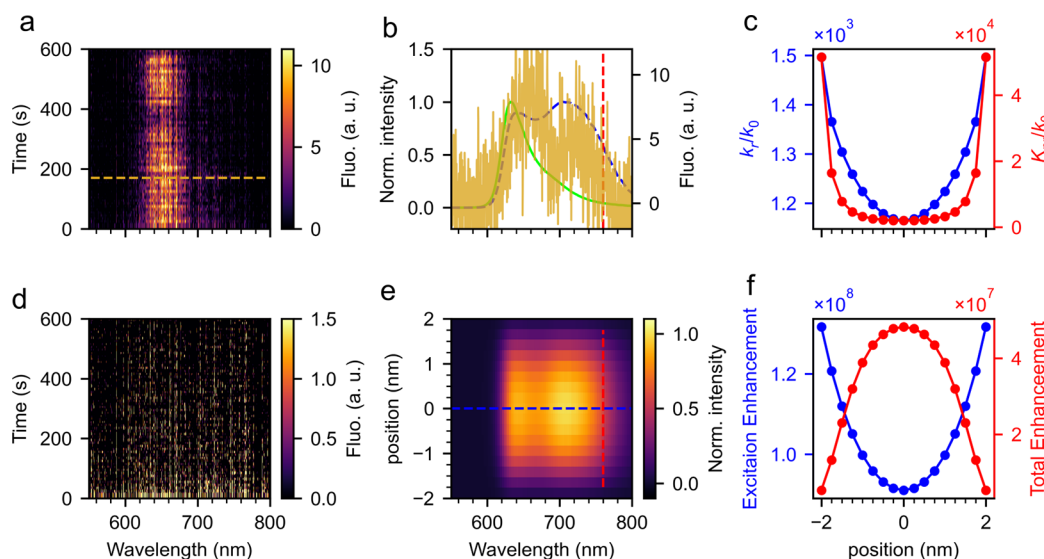
Figure 3. Two-photon-excited fluorescence enhancement in the plasmonic hot spot of an end-to-end gold nanorod dimer. (a and d) Real-time spectra of a gold nanorod dimer with (a) and without (d) the presence of 100 nM ATTO 610 in solution. (b) Comparison of the measured spectrum (orange, corresponding to the recorded time of the orange dashed line in panel a) with the spectrum of free ATTO 610 dye in solution (green solid) and the simulated enhanced spectra (blue dashed, corresponding to the blue dashed line in panel e) in the hot spot. (e) Simulated emission spectra of an ATTO 610 molecule at different positions along the main axis of the gold nanorod dimer in the gap. (c) Calculated radiative (blue) and nonradiative (red) enhancement factor as functions of the position in the hot spot and (f) respective excitation (blue) and total emission (red) enhancements. The vertical red dashed lines in panels b and e represent the wavelength of the femtosecond laser.
