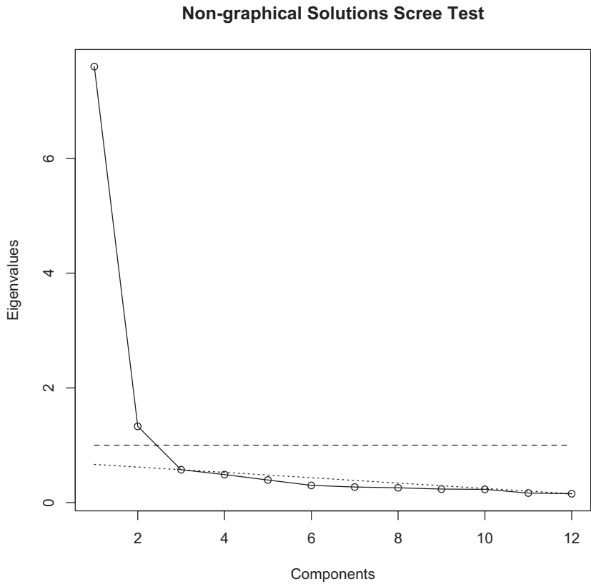
Figure 2. Non-graphical Solution Scree Test.
