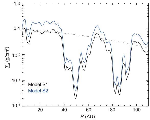
Figure a2 (Color online) Dust surface densities of model S1 (black solid line) and model S2 (blue solid line). The grey dashed line represents the initial density profile used in the iteration process, see sect. 3.3.
