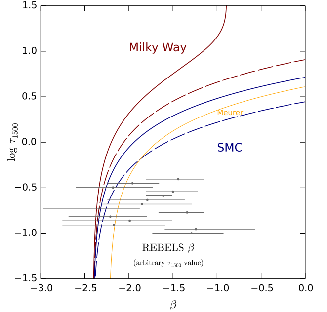
Figure 1. Relation between optical depth at 1500Å, \tau_{1500} , and UV spectral slope, \beta , often referred to as the attenuation curve, for the Milky Way (red curves) and SMC (blue) for a slab (solid) and spherical (dashed) geometry with \zeta = 2 (i.e., the dust scale height is twice the stellar one). Also shown for reference is the empirical Meurer et al. (1999) relation (orange) \tau_{1600} = 4.43 + 1.99\beta . The \beta values for the 14 REBELS sources with 158μm continuum detections are shown by grey points/lines at arbitrary \tau_{1500} values.
