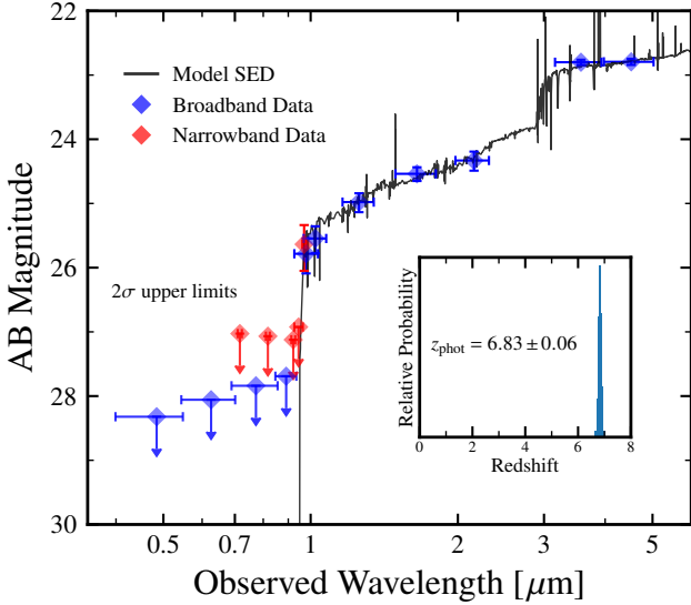
Figure 4. Results from fitting the optical and near-IR (0.3–5 \mu m) photometry of COS-87259 with BEAGLE (Chevallard & Charlot 2016). Broadband measurements are shown with blue diamonds while the narrow/intermediate-band data from HSC are shown in red. The best-fitting model SED is shown with the black curve. The redshift of this source is highly favored at z > 6 (>99.99% confidence; see inset panel) due to the sharp flux discontinuity between the HSC ib945 and nb973 bands. Because the Lyman-alpha break is expected to lie in the small wavelength range between these two bands ( \Delta\lambda = 250 \text{ \AA} ), the redshift is precisely constrained to z = 6.83 \pm 0.06 . We compare the fits of forced low-redshift solutions in Fig. 5.
