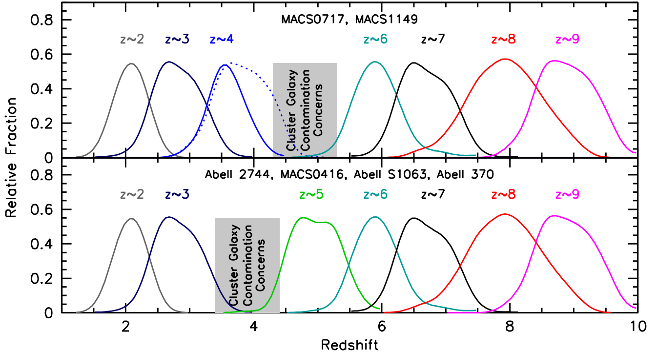
Figure 2. The expected redshift distributions of our z \sim 2, 3, 4, 5, 6, 7, 8 , and 9 selections over the HFF clusters for the two higher-redshift ( z \sim 0.55 ) clusters from the HFF program (MACS0717 and MACS1149: upper panel) and four HFF clusters at lower redshifts ( z \sim 0.3\text{--}0.4 : A2744, MACS0416, AS1063, and A370). These redshift distributions are computed from source injection and recovery experiments (as, e.g., Bouwens et al. 2021b utilize). Due to the similar wavelength of the Lyman break in z \sim 4 and z \sim 5 galaxies to the Balmer/4000 Å break in foreground galaxies that make up the lower-redshift and higher-redshift clusters (see Figure 3), we only consider selections of z \sim 4 galaxies for the two higher-redshift clusters and only consider selections of z \sim 5 galaxies for the four lower-redshift clusters. The dotted blue line in the upper panel shows the expected z \sim 4 redshift distribution when utilizing our normal z \sim 4 selection criteria (which would be appropriate if a foreground cluster were not present in our search field).
