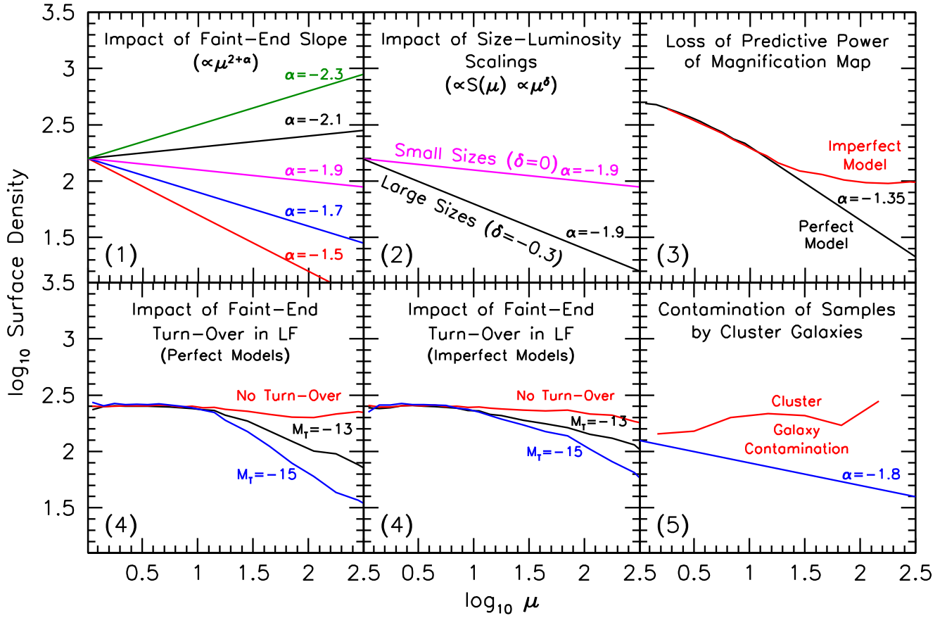
Figure 10. Schematic illustrating how the surface density \Sigma of galaxies would be expected to depend on the magnification factor \mu , as outlined in the five subsections of Section 4.1: the relevant subsection number is indicated in each panel. Five of the six panels illustrate a different issue that impacts the dependence. As shown in Section 3 of Bouwens et al. (2017; see also Broadhurst 1995; Broadhurst et al. 2005), the observed surface densities are expected to vary as \mu^{2+\alpha}S(\mu) where S(\mu) is the completeness of faint selections as a function of magnifications \mu . The numbering here and in the figure corresponds to the numbering in Section 4.1. (1) The upper-left panel shows the expected dependence on the faint-end slope \alpha of the LF (with assumed \alpha 's indicated on the figure), while (2) the upper-middle panel shows the expected dependence on different size–luminosity relations, while keeping the assumed faint-end slope \alpha fixed to -1.9 . Different size–luminosity relations translate into different magnification-dependent selection efficiencies S(\mu) , which we model as \mu^\delta . The large size–luminosity relation shown here relies on the S(\mu) \propto \mu^{-0.3} dependence found by Oesch et al. (2015), i.e., equivalent to \delta = -0.3 in the chosen parameterization, while the small size–luminosity relation assumes that sources are unresolved (e.g., Bouwens et al. 2017a; Kawamata et al. 2018; Bouwens et al. 2021a, 2022), resulting in a magnification-independent selection efficiency, i.e., \delta = 0 . (3) The upper-right panel shows the expected flattening to the \Sigma vs. model \mu relationship, due to a breakdown in the predictive power of the models (see Figure 5 of Bouwens et al. 2017c, where this result was previously shown) and assumes a faint-end slope of -1.35 to the UV LF. (4) The lower-left and -center panels present the impact of a turnover in the UV LF at the faint end, with no faint-end turnover (red), a turnover M_T at -15 mag (black), and a turnover M_T at -13 mag (blue), respectively. The lower-left panel shows the dependence assuming perfect recovery of the magnification factor, while the lower-center panel shows the dependence in a more realistic scenario where the magnifications are uncertain. (5) The lower-right panel contrasts the expected dependence for z \sim 5 galaxies (assuming a faint-end slope \alpha of -1.8 ) with that expected including large numbers of foreground galaxies from the clusters A2744 and MACS0416. The selection efficiency is assumed to be independent of magnification, i.e., \delta = 0 , except in the upper-center panel.
