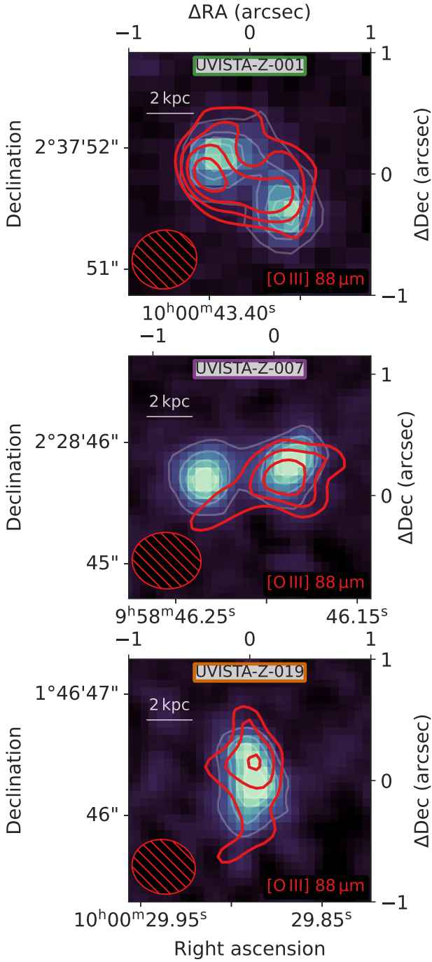
Figure 8. HST images of the rest-frame UV (in the JH_{140} band; Section 2.3) overlaid by contours of the [\text{O III}] 88\ \mu\text{m} line (achieving a \sim 0.4'' resolution with natural weighting; see Table 2) of UVISTA-Z-001 (top panel), UVISTA-Z-007 (middle panel) and UVISTA-Z-019 (bottom panel). Red [\text{O III}] contours are drawn from 3\sigma and going up in steps of 1\sigma . The top left indicates a physical scale of 2 kpc. Beam sizes for [\text{O III}] are indicated in the bottom left.
