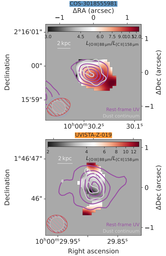
Figure 9. Line ratio maps of the [\text{O III}] 88\ \mu\text{m} and [\text{C II}] 158\ \mu\text{m} lines for COS-3018555981 (top panel) and UVISTA-Z-019 (bottom panel), where imaging parameters have been chosen to match beam sizes (see Table 2). Light grey contours are drawn for the dust continuum (at \sim 160\ \mu\text{m} , with natural weighting scheme; Section 5.6 for details), starting from 3\sigma and going up in steps of 2\sigma . Purple contours are drawn for the HST imaging (Section 2.3) of the rest-frame UV (convolved to match the dust continuum PSF), starting from 5\sigma and going up in steps of 5\sigma . Beam sizes are indicated in the bottom left (partially hiding a foreground source in the HST imaging of COS-3018555981); the top left indicates a physical scale of 2 kpc. There is tentative evidence for spatial variation in the [\text{O III}]/[\text{C II}] ratio, including a gradient with the lowest [\text{O III}]/[\text{C II}] values seeming to align with the location of the dust emission in COS-3018555981.
