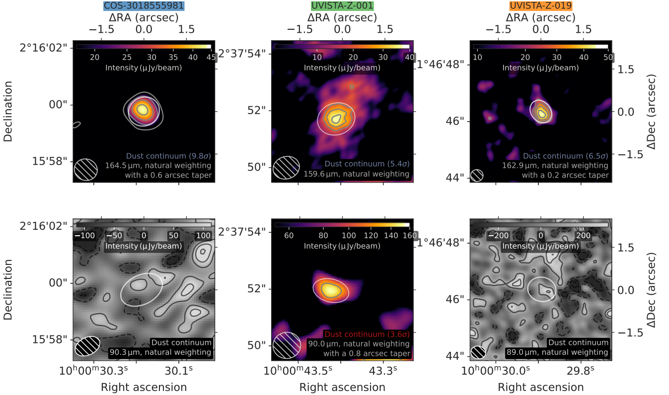
Figure 1. Naturally weighted dust continuum maps of COS-3018555981 (first column), UVISTA-Z-001 (second column), and UVISTA-Z-019 (third column); beam sizes are indicated in the bottom left. Top row: clear detections at \lambda_{\text{emit}} \sim 160 \mu\text{m} (imaged with varying degrees of taper; see Sections 2.2.2 and 3.1). Grey contours show subsequent significance levels in steps of 2\sigma (COS-3018555981) or 1\sigma (UVISTA-Z-001 and UVISTA-Z-019), starting at 3\sigma . White ellipses show the two-dimensional Gaussian fit obtained by IMFIT procedure in CASA . Bottom row: (non-)detections at \lambda_{\text{emit}} \sim 90 \mu\text{m} . Contours are the same as the top row for UVISTA-Z-001, otherwise solid (dashed) grey lines show positive (negative) 1\sigma , 2\sigma , and 3\sigma contours and white ellipses show the aperture used for determining a flux density upper limit (Section 3.1). Since there is significant extended emission at \sim 160 \mu\text{m} in UVISTA-Z-001, the white ellipses show the aperture used to measure the flux of the compact component in both the top and bottom panels (Section 3.1).
