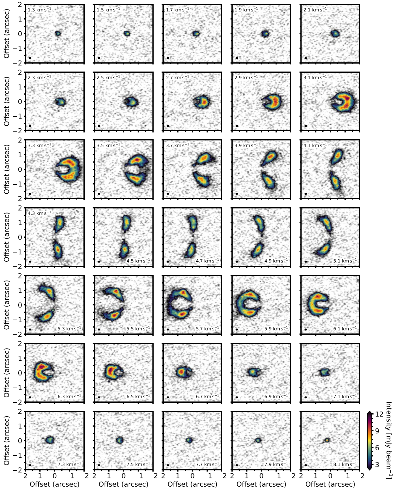
Figure 8. Channel maps showing the ^{13}\text{CO } J = 2-1 emission. The color map starts at 5\sigma . The synthesized beam is shown in the lower-left corner of each panel. An interactive version of the figure made with TRIVIA is available. Controls at the top allow the user to zoom, pan, and rescale the images. The controls at the bottom include a slider and play/stop buttons to cycle through the channel maps. Placing the cursor in the image will display the positional offset and intensity.
