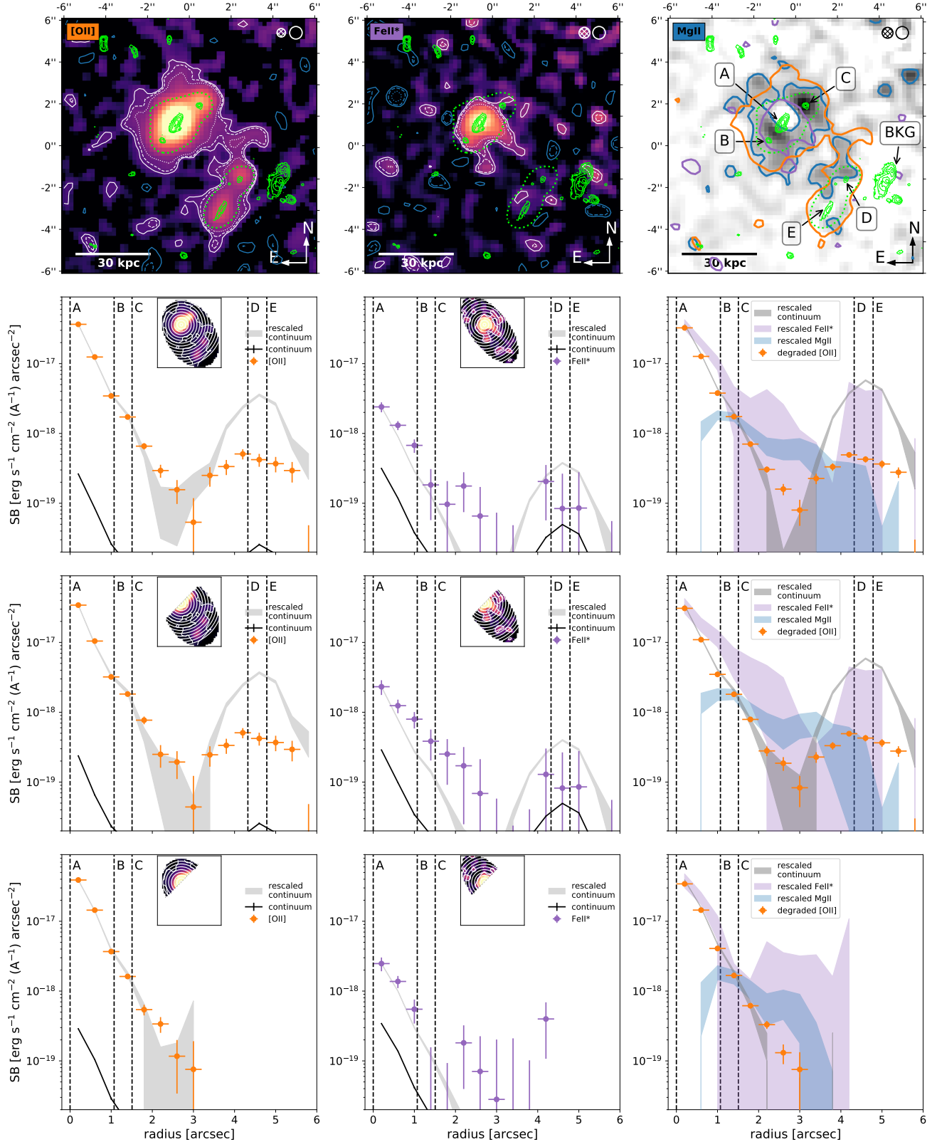
Fig. 7. [O II] and Fe II* spatial properties. First column: [O II] NB image (top, Sect. 5.1). Legend is the same as in Fig. 3a. The 1\sigma level corresponds to a SB of 2.5 \times 10^{-19} erg s -1 cm -2 arcsec -2 . Bottom panels: total and directional (below and above the [A,B,C] axis) azimuthally averaged radial SB profiles centered on galaxy A (from top to bottom, respectively, see also insets for illustration) of the [O II], [O II] continuum and rescaled [O II] continuum (orange, black and gray, respectively) emission. The radial positions of other group members with respect to galaxy A are indicated by the vertical dashed lines. Second column: same as first column but for Fe II* (purple). Third column: comparison of the Mg II, [O II] and Fe II* 2\sigma significance level contours (blue, orange, and purple, respectively) superimposed on the Mg II NB image (top). Bottom panels: show a comparison of the radial SB profiles where the Fe II* profile (shaded purple) has been rescaled to the [O II] profile at the SB peak and Mg II (shaded blue) at the position of galaxy C (Appendix D). For this plot the [O II] map was degraded to the resolution of the Mg II emission (Sect. 5.1).
