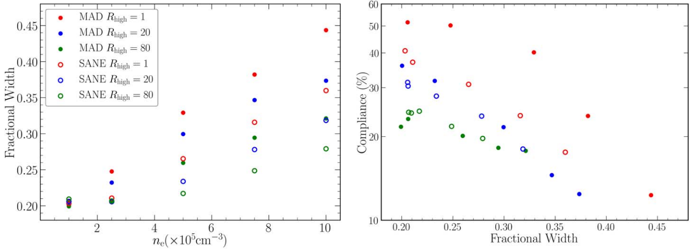
Figure 8. Left: the fractional width of the ring of emission in the average image of each simulation in Set A. Right: the anticorrelation between the fractional width and compliance fraction in the simulation set A.
