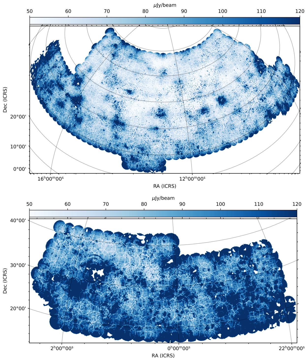
Fig. 2. The noise variations in the two regions covered by LoTSS-DR2 with the coverage of the 841 individual pointing outlined. The RA-13 (top) and RA-1 (bottom) regions span 4178 and 1457 square degrees and have median rms values of 74\mu\text{Jy}/\text{beam} and 106\mu\text{Jy}/\text{beam} respectively. Failed facets (white regions) are generally caused by either poor ionospheric conditions or dynamic range issues around bright sources such as 3C 48 and 3C 196.
