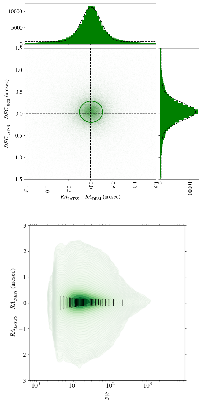
Fig. 8. The astrometric accuracy of the LoTSS-DR2 radio wavelength positions. The top plot shows the offsets in RA and DEC for compact, deconvolved LoTSS sources from their DESI Legacy Imaging Surveys counterpart. The histograms show the distribution of offsets as a function of RA and DEC and the fitted Gaussian (plus a constant) functions have \sigma_{RA} = 0.22'' and \sigma_{DEC} = 0.20'' and are centred at offsets of 0.02'' in RA and 0.05'' in DEC. The constant in the fitted function is included to allow for possible mismatches in the association of LoTSS and DESI sources. The bottom plot shows the distribution of RA offsets as a function of signal to noise with the total length of the error bars corresponding to the standard deviation of the Gaussian (plus a constant) function fitted to the sources in that particular signal to noise bin. The signal to noise bins are selected such that they contain an equal number of sources.
