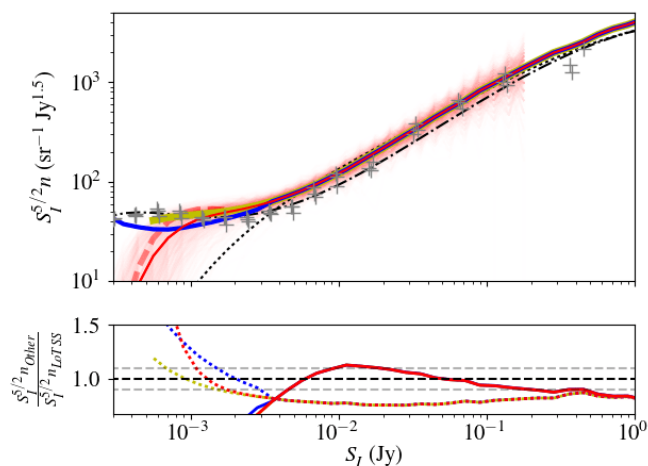
Fig. 20. The 120-168 MHz Euclidean normalized differential source counts derived from LoTSS-DR2 PYBDSF catalogues. The completely uncorrected source counts are shown in the top panel with transparent red solid lines showing those derived from individual pointings for flux density bins where at least 90% of the pointings contain more than 10 sources. The opaque red solid line shows the combined uncorrected counts from all mosaics thus spanning the entirety of LoTSS-DR2. The solid yellow line shows the counts produced from only highly complete (at least 90% of sources detected at a given threshold) LoTSS-DR2 regions (Method One in Sect. 3.8). The solid blue line shows counts that are corrected for incompleteness using the simulations that are detailed in Sect. 3.6 (Method Two in Sect. 3.8). The simulations where sources are injected according to the Mandal et al. (2021) source count fit and recovered with PYBDSF are shown by the thick red dashed line. The black dashdot line shows the Mandal et al. (2021) fitted counts, the black dotted line shows the Intema et al. (2017) fitted counts and the grey +’s show the sources counts of the three different fields analysed by Mandal et al. (2021) that were combined in their fitting. Poisson errors on our counts are too small to be seen but the variation amongst the different mosaics (transparent red lines) reflects the level of agreement between different regions in LoTSS-DR2. In the bottom panel we show the ratio of the Intema et al. (2017) (solid lines) and Mandal et al. (2021) (dotted lines) source counts compared to those from LoTSS-DR2 (colour scheme the same as the top panel). The black and grey horizontal dashed lines mark a source counts ratio of 1.0 and 1.0 \pm 0.1 respectively.
