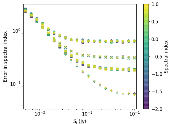
Fig. 17. The simulated measurement error in spectral index as a function of S_l where the marker colour indicates the simulated spectral index ( \alpha ). The simulation assumes an independent 10% (circles), 5% ( \times 's), 3% (boxes), or 1% (+'s) flux density alignment uncertainty on each in-band image which are added in quadrature to the image noise values of 220, 195 and 190 \mu\text{Jy}/\text{beam} for the 128.0, 143.7 and 160.2 MHz in-band images respectively. The spectral index errors were calculated by simulating 1000 sources at each flux density, spectral index and flux density alignment uncertainty and computing the standard deviation of the recovered spectral index values.
