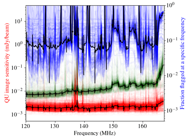
Fig. 22. The sensitivity of our Stokes Q and U image cubes as a function of frequency is shown in green (4'' resolution) and red (20'' resolution). The fraction of data flagged in our LoTSS-DR2 datasets as a function of frequency is the key contributing factor to the variation in noise levels and is shown in blue. For each plot the individual coloured lines show the properties of each image cube or dataset where the black line, and corresponding errors, show the median values at a particular frequency plus/minus the standard deviation amongst the 841 different LoTSS pointings.
