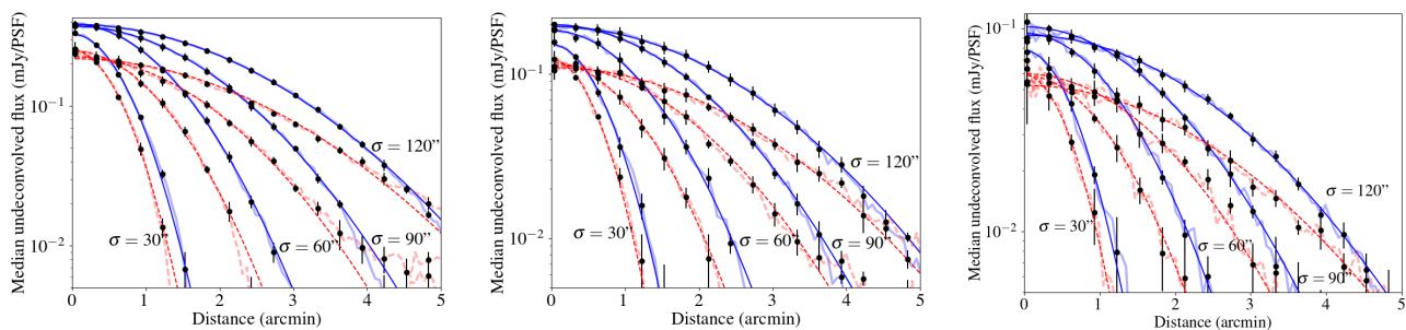
Fig. 11. The recovery of unmodelled flux density in the LoTSS-DR2 pipeline for highly extended sources. Four Gaussian profiles (with standard deviations of 30, 60, 90, 120 '' ) with different peak brightness levels (10 \mu Jy/pixel, 5 \mu Jy/pixel and 2.5 \mu Jy/pixel from left to right) are each injected 5 times into LoTSS-DR2 uv -data prior to a direction dependent calibration step using a sky model that does not include their emission. The black error bars and thicker lines show the median and the standard deviation of the image brightness values as a function of distance for each of the different injected profiles. The thin solid lines are the best fit profiles to these median values. Blue lines correspond to values derived from the undeconvolved pre direction dependent calibrated image (i.e. image from Step.3 or the centre panel in Fig. 12) and the red lines correspond to the undeconvolved post direction dependent calibrated images (i.e. image from Step.5 or the right panel in Fig. 12). Overall, by integrating the simulated and recovered signal out to five standard deviations from the Gaussian centroid we find that in this worst-case scenario typically 60 \pm 6\% of injected but completely unmodelled flux density is recovered after direction dependent calibration.
