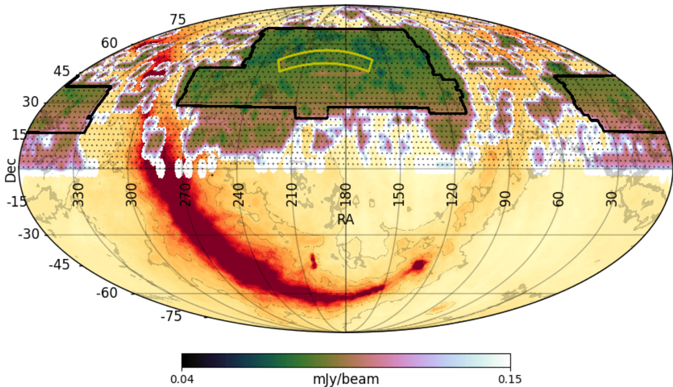
Fig. 1. The status of the LoTSS observations as of April 2021 and the approximate current sensitivity coverage (accounting for station projection and typical sensitivities achieved to date) overlaid on the Haslam et al. (1982) 408 MHz all-sky image (corresponding to yellow to deep red colours, with associated contours). The yellow and black outlines show the LoTSS-DR1 and LoTSS-DR2 areas respectively and the small black dots show the 3168 LoTSS grid positions. LoTSS-DR1 included 63 pointings, LoTSS-DR2 includes 841 pointings; we have fully observed 1623 pointings including those of DR2, a further 154 pointings are partly observed and observations still need to be conducted for 1391 pointings to complete the survey.
