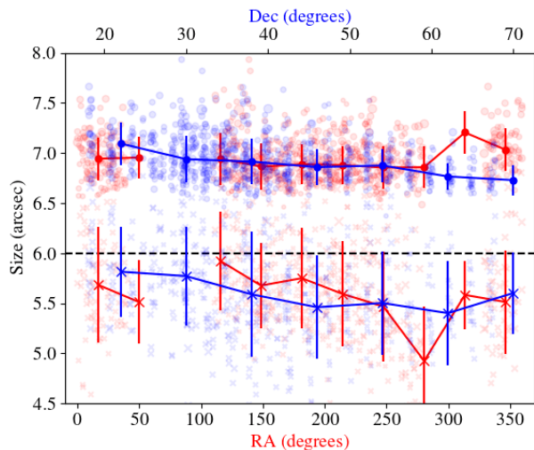
Fig. 7. The compact source and synthesized beam size as a function of right ascension (red, lower x-axis) and declination (blue, upper x-axis). The synthesized beam (transparent ‘x’ symbols) size for each LoTSS-DR2 pointing is the average of the major and minor FWHM of a fitted Gaussian. The compact source size (transparent circles) is the median of the average of the major and minor FWHM of the compact sources (according to Eq. 2) with S/N greater than 20 in each mosaic. The marker sizes are proportional to the image rms (accounting for the flagging fraction and integration time) which is a proxy of data quality. The solid lines and larger markers show the median of both the synthesized beam (solid ‘x’ symbols) and compact source (solid circles) sizes as a function of right ascension (red) and declination (blue) and the errors show the corresponding standard deviations. The dashed black line shows the size of the restoring beam which is kept constant over the entirety of LoTSS-DR2 and is generally larger than the synthesized beam.
