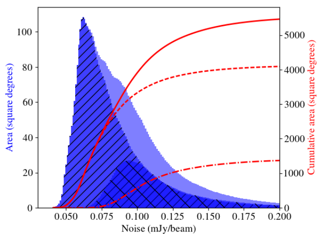
Fig. 14. The overall rms distribution of LoTSS-DR2 is shown in the light blue histogram (y-axis on the left). The contributions from the RA-13 and RA-1 regions are shown by the darker blue histograms with \ and / hatching respectively. The rms distributions of the two regions are approximately equal above 0.1 mJy/beam but otherwise the RA-13 region is on average higher declination and therefore generally more sensitive than the RA-1 region. The median and mean of the rms are 83 \mu\text{Jy/beam} and 95 \mu\text{Jy/beam} over the entire LoTSS-DR2 region where 90% and 95% is below 140 and 170 \mu\text{Jy/beam} respectively. The solid red line shows the cumulative area of the entire LoTSS-DR2 region with an rms noise below a given value with the dashed and dashdot lines showing the same but for the RA-13 and RA-1 regions (y-axis on the right).
