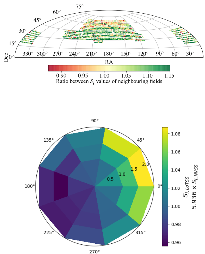
Fig. 9. The top panel shows the ratios between S_I measurements of isolated, compact, deconvolved sources, within 30% of the primary beam power level in overlapping LoTSS-DR2 pointings that are predominantly separated in declination. These are projected onto the sky with the position being the mean position of the overlapping pointings and the colour scale indicates the best fit ratio between the S_I values. The bottom panel shows the median LoTSS to NVSS S_I ratios (divided by 5.936 to centre on unity) for different segments of individual fields averaged together for all LoTSS-DR2 fields with a declination less than 50^\circ . Here 0^\circ is North, the angle increases from North through West and the segments extend up to 2^\circ from the pointing centres.
