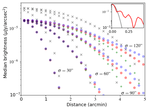
Fig. 10. The recovery of simulated Gaussian skymodels of varying width and brightness that are injected into calibrated uv -data. The red points show the brightness as a function of distance from the centroid of the simulated skymodels convolved by a Gaussian with a size that matches the restoring beam dimensions. The blue points show the profile of the emission recovered in the restored image created from the simulated uv -data. The green '+' symbols show the flux density in the corresponding model image created during the deconvolution of the simulated uv -data that has been convolved with a Gaussian with a size that matches the restoring beam. The 'x' symbols show the flux density in the undeconvolved image of the uv -data. The different profiles show the different values of standard deviations of the injected Gaussian profile. When the emission is deconvolved the model injected into the data matches the profile and flux density of the emission recovered in the restored image. However, when the emission is not fully deconvolved (e.g. in the undeconvolved image or in the restored image where the emission becomes very faint) the apparent flux density can be either severely overestimated or underestimated and can be highly misleading due to the mismatch in area of the synthesised (red) and restoring beams (grey) which are shown in the inset.
