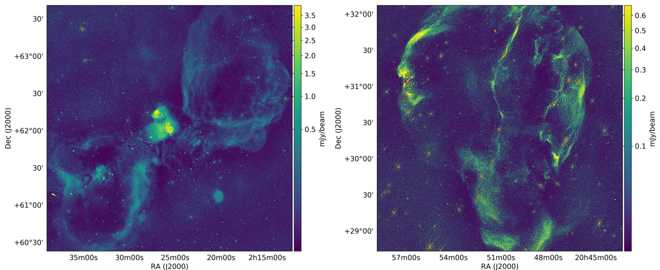
Fig. 23. LoTSS mosaics showing the W3/W4/HB3 star forming region (left) and the Cygnus loop supernova remnant at an angular resolution of 6'' . The mosaics have sensitivities of approximately 120\mu\text{Jy}/\text{beam} and the emission, which is deconvolved, from each of these Galactic regions spans over 12 million 1.5'' \times 1.5'' pixels. The calibration of these complex regions was done with a modified version of the pipeline used for LoTSS-DR2 which provided more stability whilst still allowing us to calibrate in 45 different directions for each individual pointing that makes up these mosaics (see Sect. 5.2 for details).
