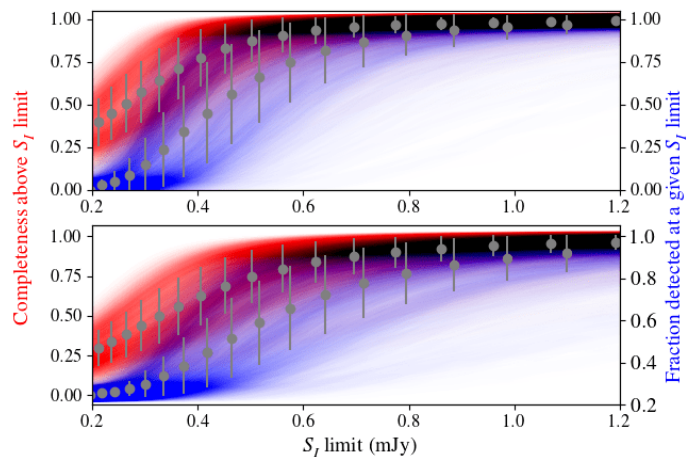
Fig. 16. The point source completeness, or fraction of simulated sources detected above some S_l limit, of LoTSS-DR2 for genuinely point-like sources (top) and for real point-like sources as defined from their recovered deconvolution models (bottom). Each red line shows the completeness derived from approximately 370,000 sources that are injected into each of the 841 DR2 mosaics through a series of 10 simulations with realistic source density and flux density distributions. The overlaid grey points represent the mean between the different mosaics weighted by the area covered by the mosaics and the error bars show \pm the standard deviation of the different mosaic values. Due to the number of sources injected into the maps the Poisson errors are negligible by comparison. The fraction of sources detected at a given flux density are also shown with blue lines where grey points again show the corresponding weighted mean values as a function of flux density.
