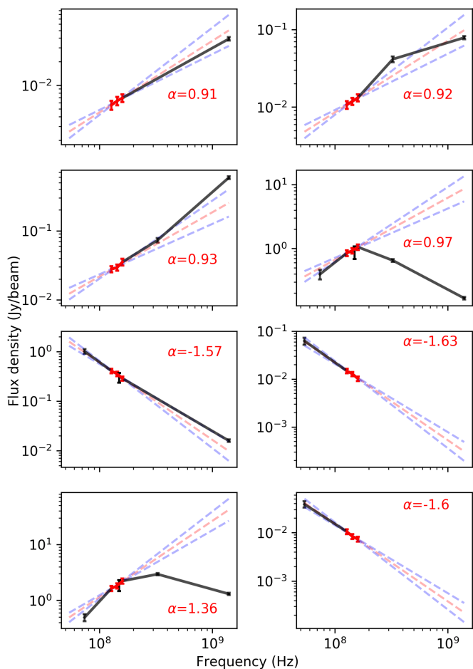
Fig. 19. Examples of sources with extreme in-band LoTSS spectral indices. The in-band LoTSS measurements are shown in red where the red dotted line shows the fitted \alpha (values of \alpha are displayed on the panels) and the blue dotted lines show the fitted \alpha \pm 0.2 . The black points show measurements from LoLSS, VLSSr, TGSS, WENSS and NVSS where available. Clockwise from top left, the sources shown are: ILTJ004259.17+233517.1, ILTJ084911.00+403231.2, ILTJ101731.34+434312.5, ILTJ113903.61+583040.5, ILTJ125903.65+594635.9, ILTJ082236.93+511230.0, ILTJ011755.08+320622.5 and ILTJ004259.17+233517.1.
