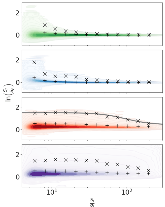
Fig. 6. The ratio of integrated flux density to peak brightness as a function of signal to noise for populations of simulated and real LoTSS-DR2 sources. The green (top) curve shows the idealised distribution where there is no bias in the detections and the noise in the integrated flux density and peak brightness are uncorrelated. The blue (second from top) curve is a population of point-like sources that were injected into images with a Gaussian noise background and catalogued using PYBDSF. The red (second from bottom) and purple (bottom) curves show populations of compact and all LoTSS-DR2 sources respectively. In each of the four distributions the + and x symbols show the 84.1 and 99.9 percentile levels in different signal to noise bins. If the data were described by a Gaussian distribution, which is only the case for the green points, these would correspond to the standard deviation and 3 \times the standard deviation respectively. The sigmoid function we have defined for separating extended and point-like sources is shown with the grey line fitted to the 99.9 percentile level of the population of compact LoTSS-DR2 sources (red points).
