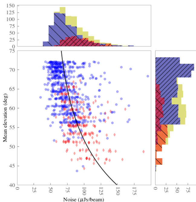
Fig. 15. The sensitivity of each individual pointing that makes up LoTSS-DR2 as a function of the mean elevation during the observation. The sensitivities are scaled to their equivalent for an 8hr run by taking into account the exact integration time and the fraction of data that are flagged. The blue points and blue histograms with \ hatchings show pointings in the RA-13 region and the red points and red histograms with / hatchings show the pointings in the lower average declination RA-1 region. The yellow histograms correspond to all pointings in both regions. The black line shows the best fit A \times \cos(90 - \text{elevation})^{-2.0} curve where A is found to be 62 \mu\text{Jy}/\text{beam} and the dependence on elevation is fixed according to the projected size of the LOFAR stations.
