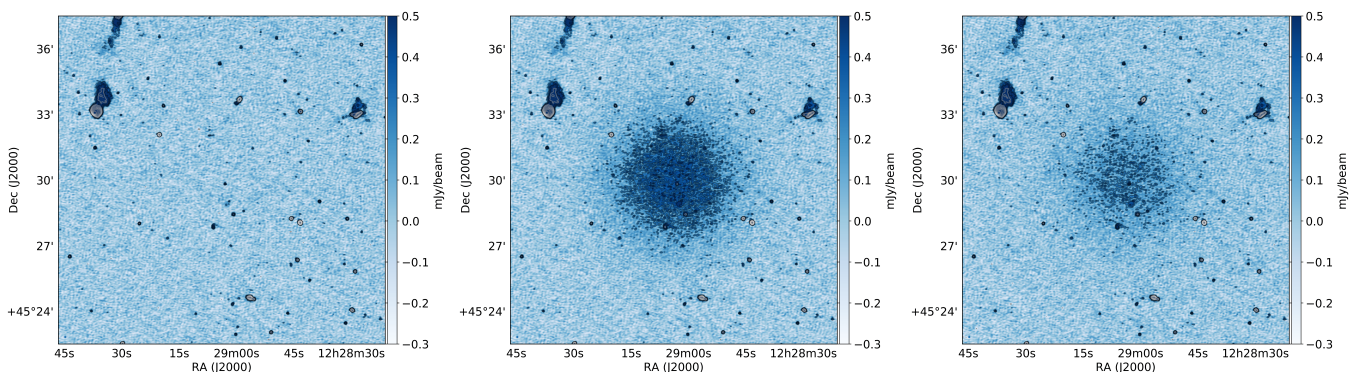
Fig. 12. An example of an injected profile, in this case the injected profile has \sigma = 120'' and a peak brightness of 10 \mu Jy/pixel. The left shows the original data. The centre shows the original data plus the injected profile that is added but not deconvolved. The right shows the resulting image after it is calibrated again but without the profile in the model and hence shows the suppression of completely unmodelled emission.
