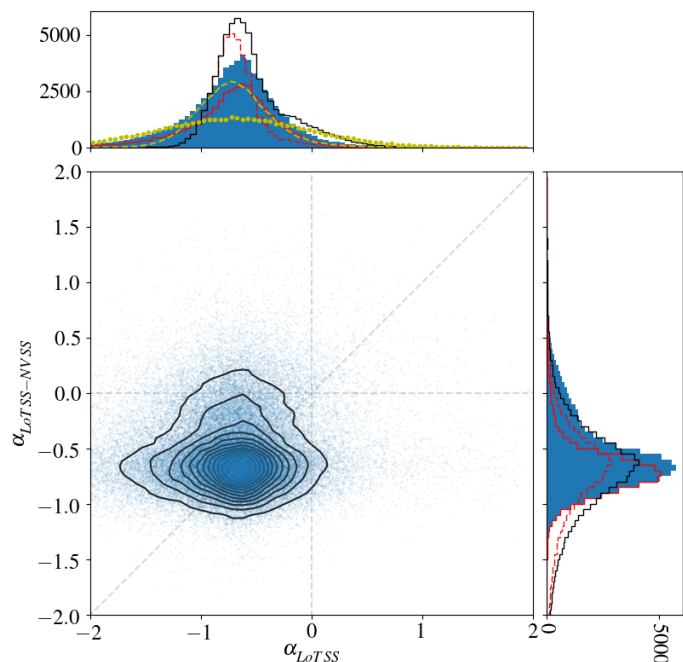
Fig. 18. The derived LoTSS-NVSS and in-band LoTSS spectral index measurements for isolated, compact, fully deconvolved LoTSS-DR2 sources overlaid with contours showing the density of points. The solid blue histograms show the in-band LoTSS spectral index distribution (top) and the LoTSS-NVSS spectral index distribution (right) for all sources where we have both measurements. The histograms outlined in black show the LoTSS-NVSS spectral index distribution of these sources overlaid on the in-band LoTSS spectral index distribution or vice versa. The solid and dashed red lines show the spectral index values derived from only bright (LoTSS S_l > 30 mJy/beam) LoTSS sources for in-band and LoTSS-NVSS (top) and LoTSS-NVSS and in-band (right) respectively. The dotted and the dashed yellow histograms (top) show the results from simulations where the LoTSS-NVSS spectral index values of bright (LoTSS S_l > 30 mJy/beam) sources, and associated errors, are used to simulate LoTSS in-band flux densities which are then fitted with a power law to give a spectral index. Here flux densities for each band and source are extrapolated from the LoTSS-NVSS spectral index and LoTSS continuum measurement plus a random error drawn from a Gaussian with a standard deviation equal to 10% (dotted) or 3% (dashed) of the flux density (mimicking a flux density scale alignment uncertainty) added in quadrature to the statistical uncertainty from the PYBDSF estimation of noise local to the source.
