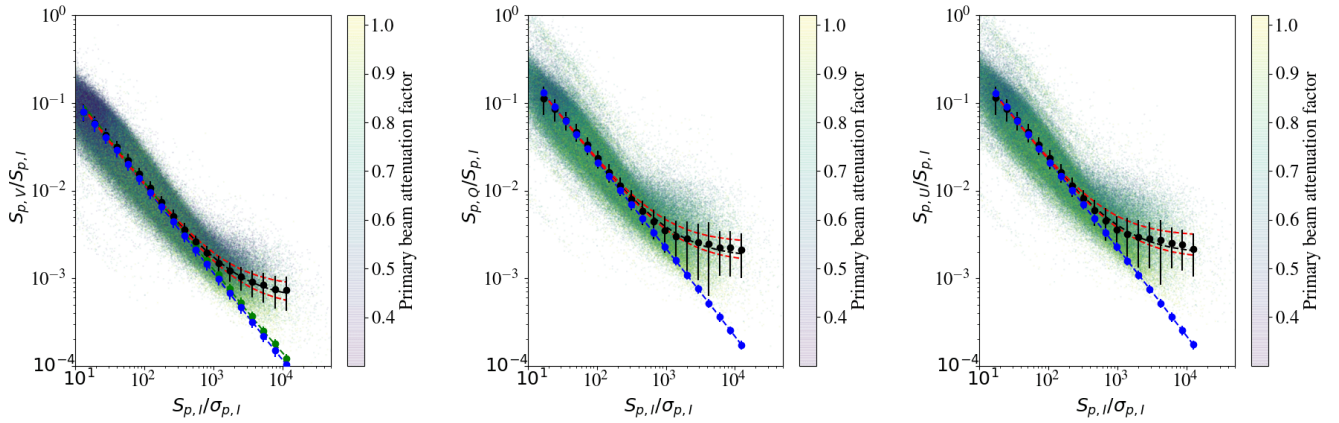
Fig. 21. The observed Stokes V (left), Q (centre) and U (right) to Stokes I maximum absolute image pixel ratios as a function of the Stokes I signal-to-noise ratio. The small points show measurements obtained from all compact, isolated LoTSS-DR2 sources with S_I > 10 mJy. The large black points show the median values in S_{p,I}/\sigma_{p,I} bins and the error bars show the standard deviation of the sources within each bin. The dashed black fitted line shows the best fit through the points which are: S_{p,V}/S_{p,I} = 1.16 \times \sigma_{p,I}/S_{p,I} + 5.7 \times 10^{-4} ; S_{p,Q}/S_{p,I} = 2.12 \times \sigma_{p,I}/S_{p,I} + 1.7 \times 10^{-3} ; and S_{p,U}/S_{p,I} = 2.1 \times \sigma_{p,I}/S_{p,I} + 1.9 \times 10^{-3} . The red dashed lines above and below the best fit line show the best fits derived when considering sources with a primary beam attenuation factor below 0.65 and above 0.65 respectively. The large blue dashed line fitted with blue dots shows the situation if the Stokes V, Q or U signals are Gaussian random noise (with pixels chosen from a region size to align the observed and simulated distributions at low S_{p,I}/\sigma_{p,I} ). In the Stokes V panel, the green dashed line fitted with green dots represents when the aperture is offset from the target and, as expected, this follows the Gaussian random noise simulation and demonstrates its validity. The real observations begin to differ significantly from the leakage-free simulations at around S_{p,I}/\sigma_{p,I} = 1,000 – above this S_{p,I}/\sigma_{p,I} we have over 23,000 measurements in Q and U and 30,000 in V (where our maps are slightly wider in area) that constrain our leakage estimates at high S_{p,I}/\sigma_{p,I} .
