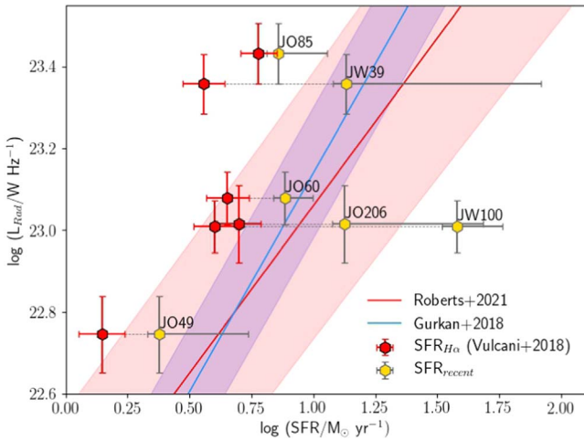
Figure 6. Integrated radio luminosity at 144 MHz vs. SFR. For each galaxy, the \text{SFR}_{H\alpha} from Vulcani et al. (2018) (red points) and \text{SFR}_{\text{recent}} (gold points; see Section 3.3), with the corresponding errors, are connected by the dashed lines. We show also the best-fit L_{\text{Rad}} –SFR relations from Gürkan et al. (2018) (blue line) and Roberts et al. (2021b) (red line). The shaded regions show the dispersion at 1\sigma around the corresponding best-fit relations.
