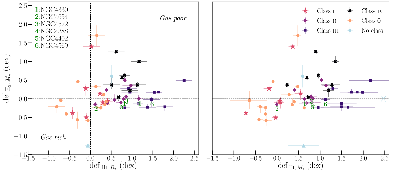
Figure 2. H_2 deficiency as a function of H I deficiency, where H I deficiency is estimated in two different ways ( \text{def}_{H I, R_*} , left-hand panel, and \text{def}_{H I, M_*} , right-hand panel). Classes refer to the H I classification from Yoon et al. (2017, see Section 3.6), based on deficiency and morphology. VCC1581, which was not detected in CO, is represented by the light-blue triangle, indicating the lower limit on its molecular gas deficiency. The x-shaped marker in the right panel indicates IC3418, which is a lower limit both in H I and H_2 deficiency (it is not present in the left-hand panel because no limit on the H I deficiency was provided by Chung et al. 2009). The numbered galaxies (green numbers are placed below the relevant markers) represent well-studied “smoking-gun” RPS galaxies, listed in the top-left corner in order of pre-to-post RP peak. There is a weak correlation between H I and H_2 deficiency: the Spearman correlation coefficient is 0.28 \pm 0.05 , with a typical p value of 0.05, for the left-hand panel and 0.36 \pm 0.04 , with a typical p value of 0.01, for the right-hand panel. Most galaxies lie in the upper-right quadrant, and are thus both H I and H_2 deficient. On average, galaxies that have H I reservoirs similar to those of field galaxies (class 0 galaxies) are least H_2 deficient, while galaxies that are H I deficient because of their lower H I surface densities (class IV galaxies) are most H_2 deficient. VERTICO galaxies undergoing RPS are relatively H_2 -rich compared to other VERTICO galaxies with similar H I deficiencies.
