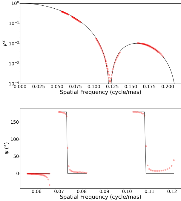
Fig. 26. Observation of \delta Vir in the L band. Top : measured squared visibilities (red) and limb-darkened model. Bottom : measured closure phases (red) and limb-darkened model. For the closure phase, the spatial frequency corresponds to the longest baseline of the triplet.
