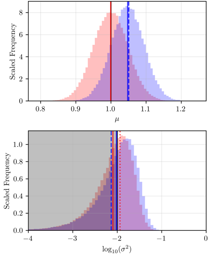
Figure 2. Distributions of the mean and variance reconstructions for a specific realization of the (u, v) -positions of simulated data points with thermal and structural variability included. In red, the distributions from an ensemble of such experiments are shown, holding the underlying mean visibility map and (u, v) positions fixed. The truth values are indicated by the vertical black lines. The average mean and variance are indicated by the vertical solid red lines. The vertical dashed red line shows the average log variance. The gray shaded region indicates the region in which the noise is subthermal. The vertical dashed blue lines indicate the \mu and \sigma^2 from the data realization used to generate the bootstrap error estimates, shown by the blue distributions and with means shown by the blue solid lines.
