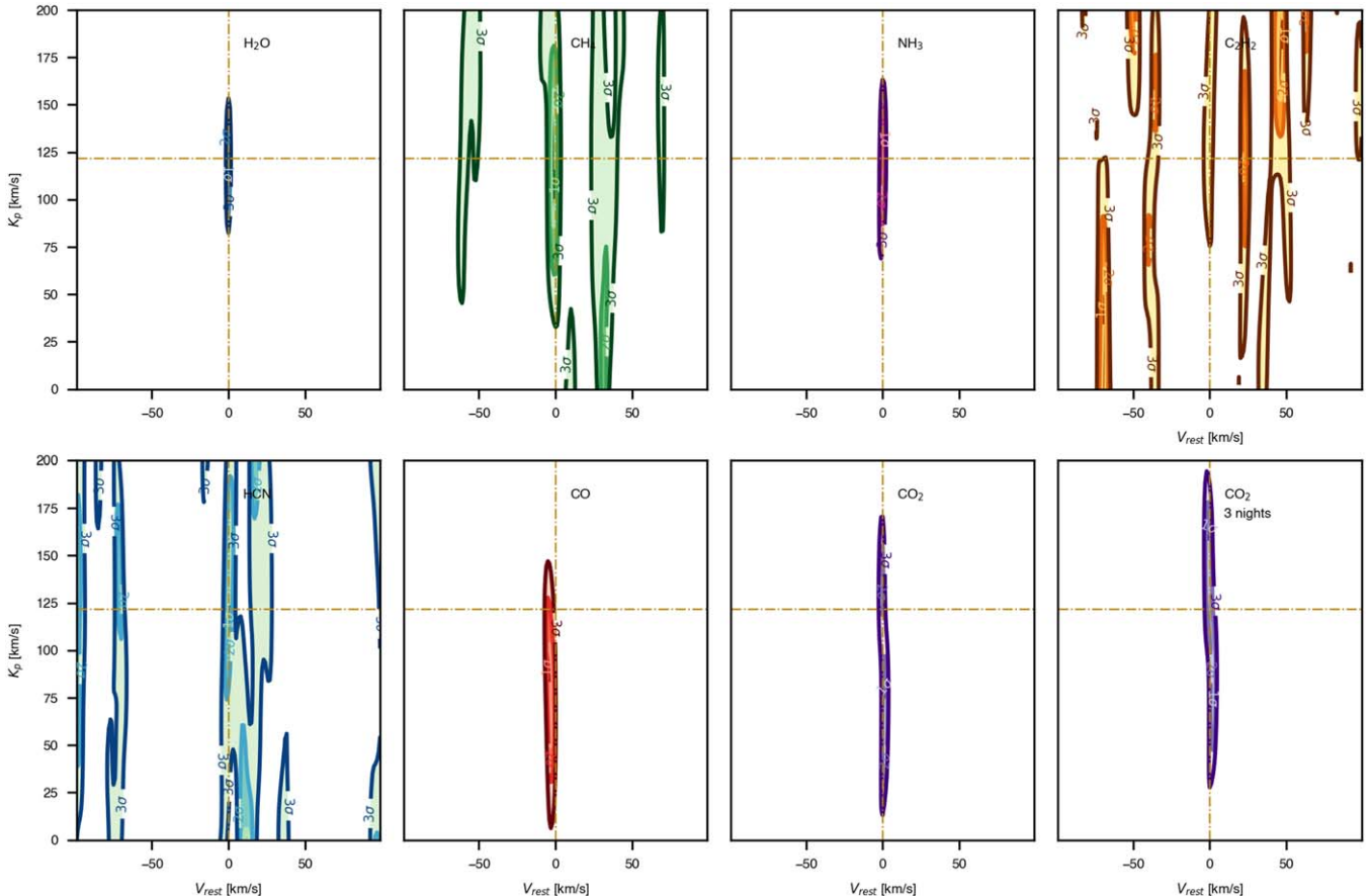
Figure 4. As Figure 2 but with v_{\text{rest}} interval between [−99, 99] km s −1 .
