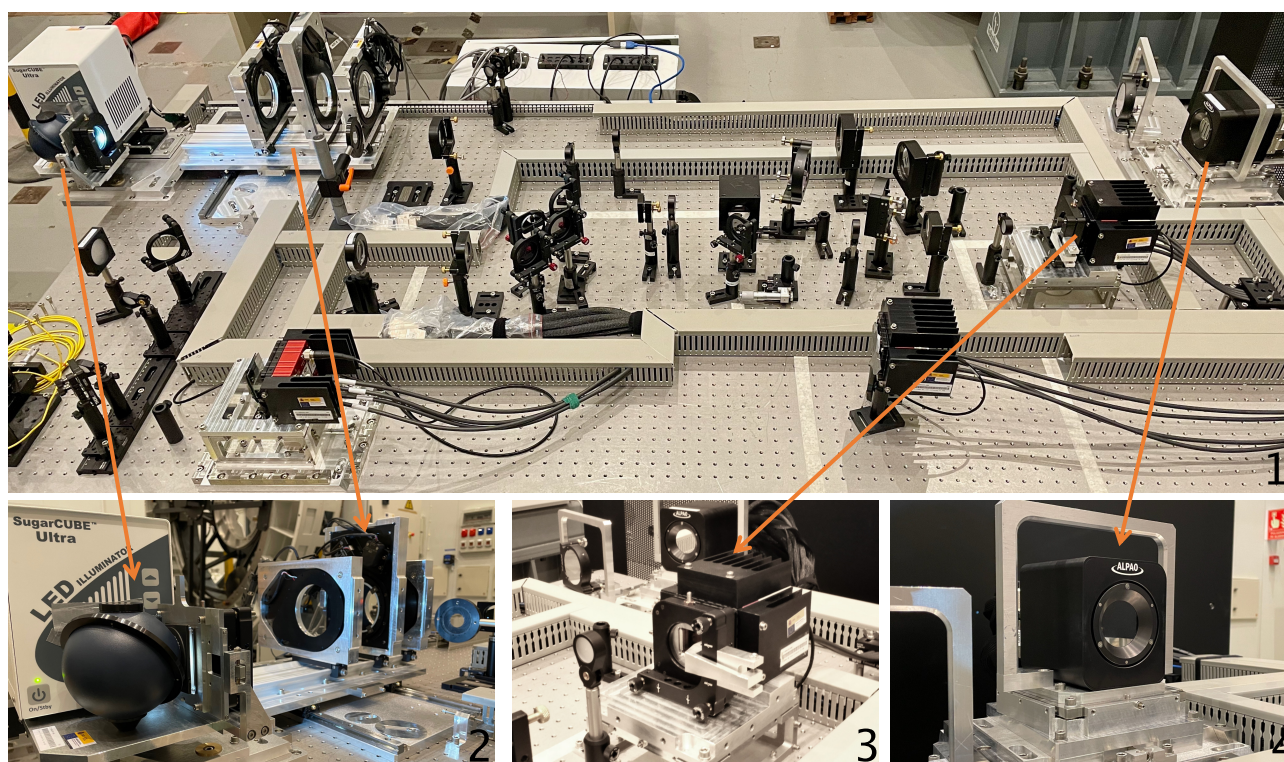
Fig. 20. MCAO test bench set-up at the IAC lab. Upper panel (label 1): current, complete set-up, while the bottom panels display a zoom-in of the main elements highlighted with arrows in the upper panel . From left to right of the bottom row , there is the extended light source and phase screens (label 2), the wavefront sensor (label 3), and the pupil deformable mirror (label 4). MCAO DMs will be added at a later stage.
