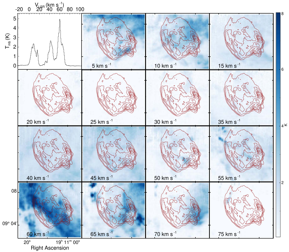
Figure 10. Channel map of the averaged main-beam temperature of ^{12}\text{CO } J=2-1 emission with a step of 5 \text{km s}^{-1} , overlaid with contours of 327 MHz radio emission. The same contours are used for the maps in the rest of the paper. The top left panel shows the spectrum averaged over the FOV.
