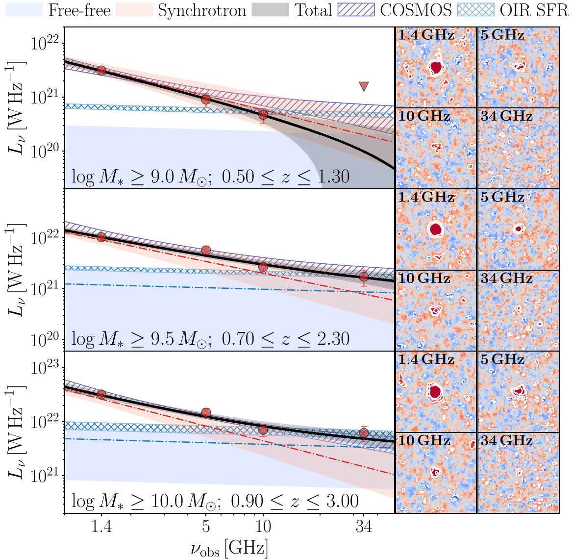
Figure 5. Similar to Figure 4, now showing the median-stacked radio spectra (left) and stacked cutouts (right) in mass-complete bins across the GOODS-N field. We detect stacked 34 GHz continuum emission in two out of three bins, at a significance of 3.4\sigma and 4.0\sigma .
