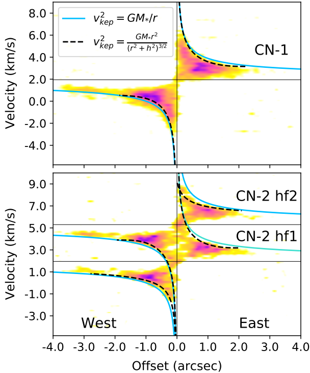
Fig. 6. Position–velocity diagrams along the semi-major axis of the disk (PA = 118.8°) for CN-1 ( top ) and CN-2 ( bottom , with two hyperfine group transitions). The offset is positive toward the east side of the disk and negative toward the west. The horizontal lines give the systemic velocity ( \sim 1.95 \text{ km s}^{-1} ), shifted for CN-2 hf2 emission to \sim 5.3 \text{ km s}^{-1} . The blue curve shows the expected Keplerian velocity curve assuming a flat disk geometry. The dashed black line is the expected Keplerian velocity considering the derived best-fit model for the vertical profile of each tracer. Both models consider a stellar mass of 0.46 M_{\odot} , as derived in Veronesi et al. (2021). The east and west sides of the disk are indicated in the bottom panel for reference.
