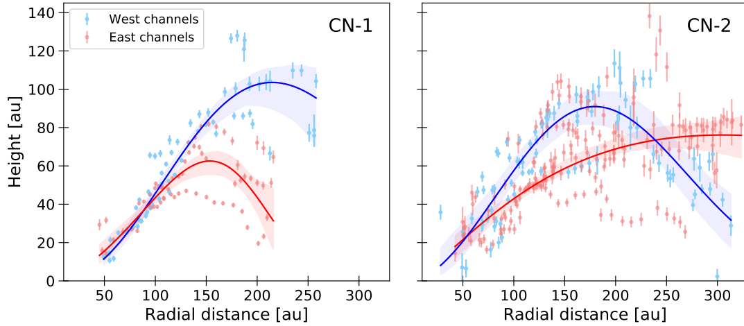
Fig. 3. Vertical location of emission from CN-1 ( left ) and CN-2 ( right ) transitions, using data obtained from the channel map analysis of the emission. The dataset is separated between the east (red dots) and west (blue dots) sides of the disk, as defined by the semi-minor axis. The solid blue and red curves trace the best-fit exponentially tapered model of each side. The colored regions show the uncertainty of the model, obtained from the spread of the posterior values from our MCMC analysis.
