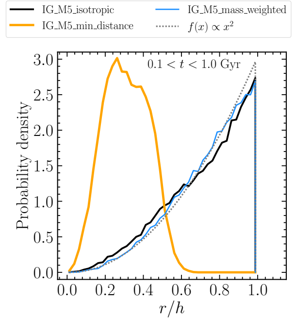
Figure B1. Probability density of the distances between stellar particles and the gas neighbours they heated in their last SN event, in units of the stellar particles' SPH smoothing length at the moment of the feedback, in the isolated galaxy simulations with resolution m_{\text{gas}} = 10^5 M_{\odot} with isotropic (black), min_distance (orange) and mass-weighted (blue) neighbour-selection methods. The SN events are selected from the time interval 0.1 < t < 1.0 Gyr. The dashed grey curve gives the probability density for f(x) \propto x^2 , corresponding to a radially unbiased distribution.
