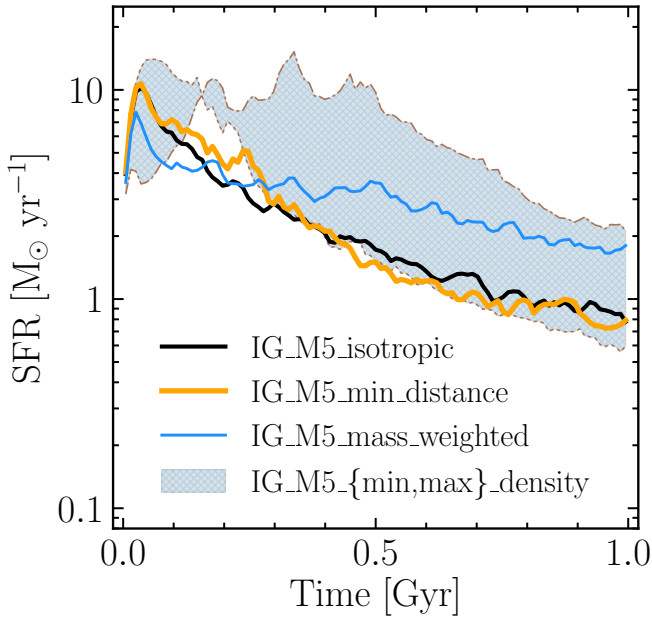
Figure 3. Star formation histories in the isolated galaxy simulations with resolution m_{\text{gas}} = 10^5 M_{\odot} with isotropic (black), min_distance (orange) and mass-weighted (blue) neighbour-selection methods for SN feedback. The hatched grey area provides an estimate of the maximum variation in the star formation rate due to the neighbour-selection strategy: its boundaries are defined by the star formation rates in the runs with the most and least efficient SN feedback: IG_M5_min_density (dashed) and IG_M5_max_density (dash-dotted), respectively.
