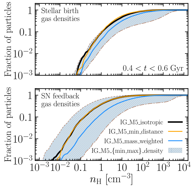
Figure 4. The cumulative distribution of stellar birth gas densities (top panel) and SN feedback gas densities (bottom panel) recorded at times 0.4 < t < 0.6 Gyr, in the isolated galaxy simulations with resolution m_{\text{gas}} = 10^5 M_{\odot} with isotropic (black), min_distance (orange) and mass-weighted (blue) neighbour-selection methods for SN feedback. The hatched grey area is constructed in the same way as in Figure 3 (i.e. using the min_density and max_density methods). Both stellar birth densities and SN feedback densities are sensitive to the method of neighbour selection.
