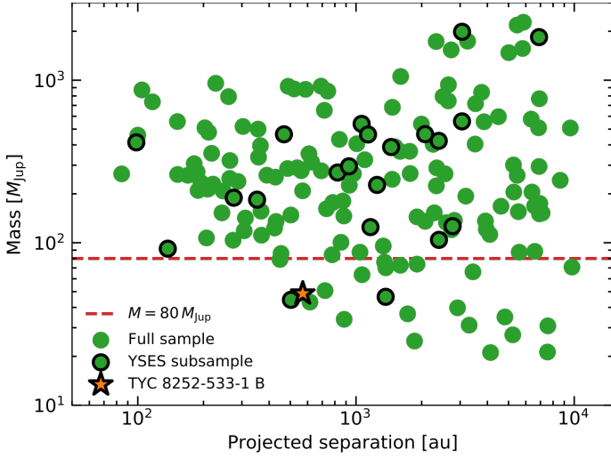
Fig. 4. Identified companion candidates to K-type Sco-Cen members II. Members of the YSES subsample are highlighted by the black outline around the marker. The orange star highlights TYC 8252-533-1 B analyzed in Sect. 4.1. The companion mass is presented as a function of projected separation in Astronomical Units. Mass conversion was performed by comparison to BT-Settl and MIST models evaluated at the system age. The dashed red line at 80 M_{\text{Jup}} indicates the threshold between brown dwarfs and stellar mass companions.
