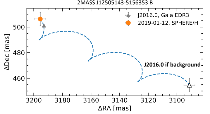
Fig. 12. Proper motion analysis of 2MASS J12505143-5156353 B. See Fig. 8 for a detailed description of the plot elements.
