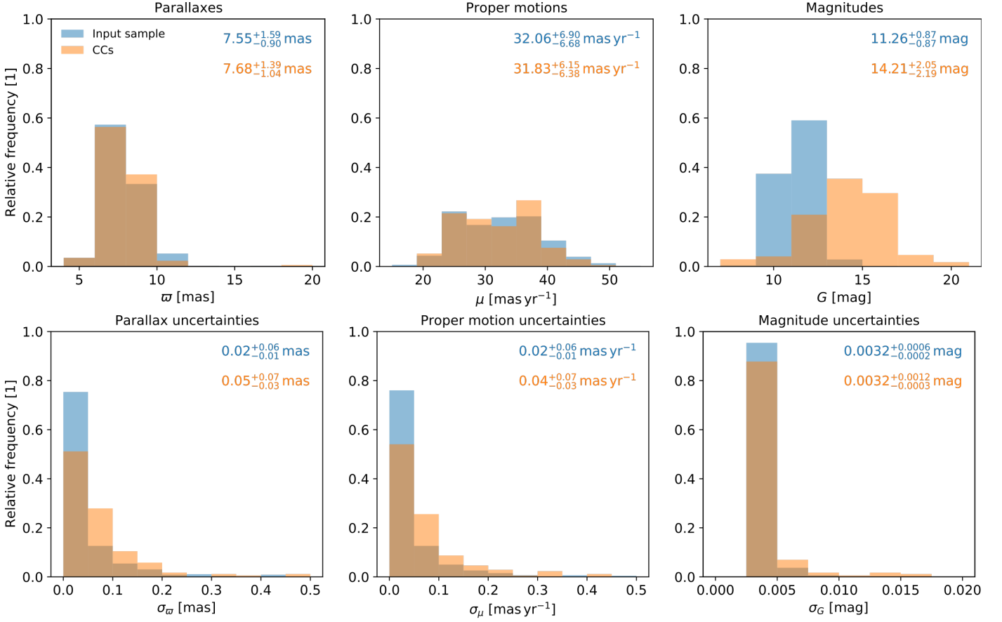
Fig. 2. Astrometric and photometric properties of the input sample and the preselected list of candidate companions (CCs). In the top panel we present the distributions of the object parallaxes, proper motions, and magnitudes from both samples. In the lower panel the uncertainties are shown. The colored values in the upper right of each panel indicate the median and the 68% confidence intervals of the associated distributions.
