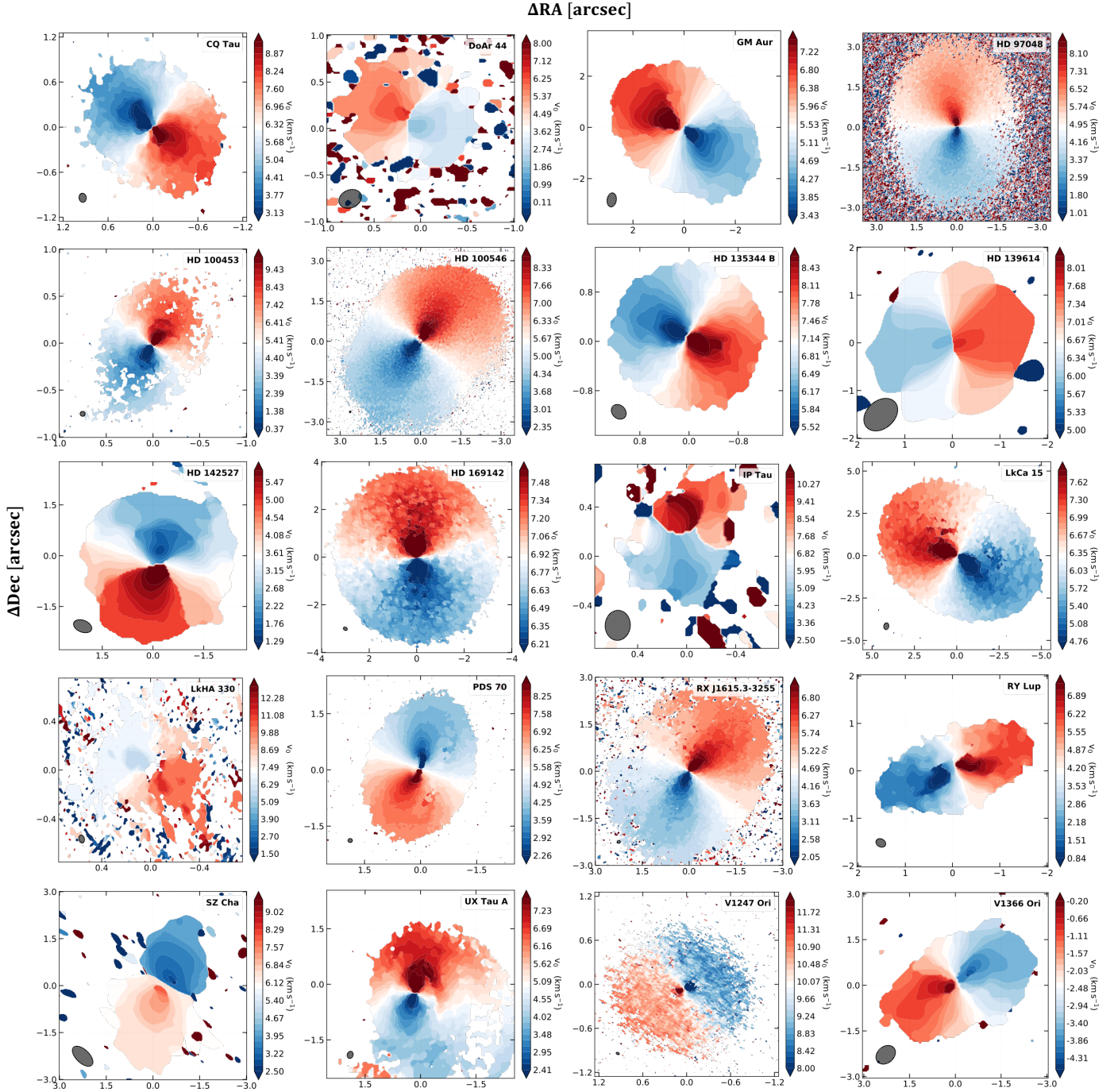
Fig. C.1: ALMA line data of our targets. We present the quadratically collapsed moment maps that were created with bettermoments by quadratic collapsing of the frequency channels. The ellipse in the lower left of each panel indicates the beam size of the observation. For all images north points up and east to the left.
