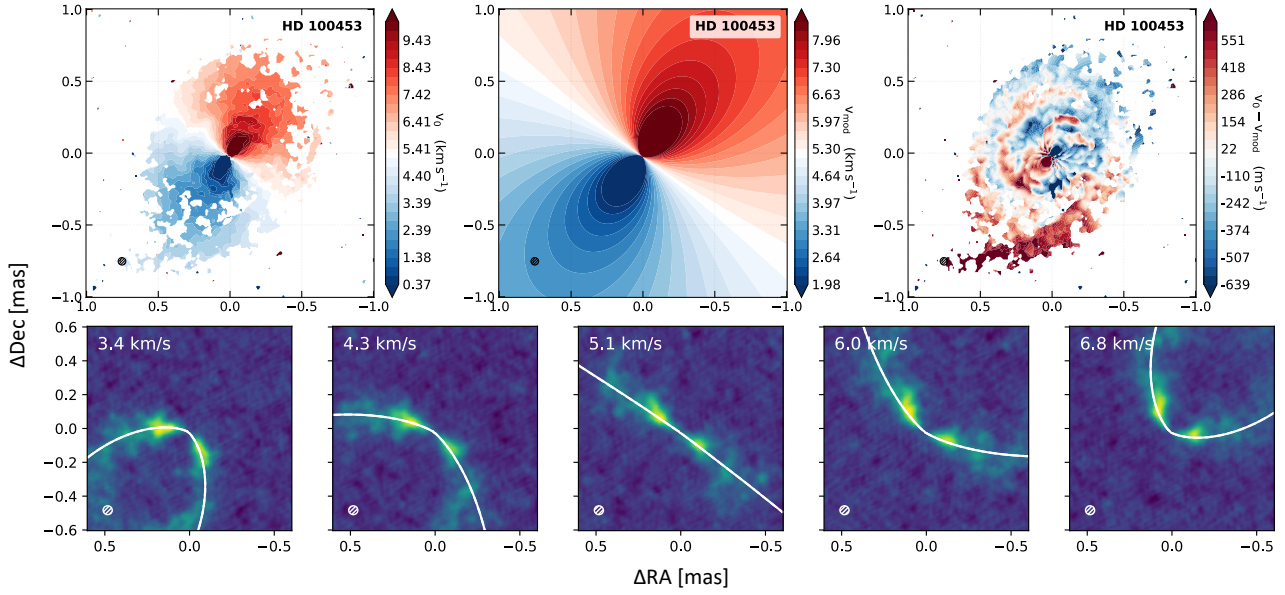
Fig. 4. Velocity maps and model fits to the ALMA CO line data of HD 100453. In all images north points up and east to the left. Top left: quadratically collapsed moment map derived with bettermoments . Top center: best-fit Keplerian disk model derived with the eddy tool. Top right: residuals after subtraction of the model from the data. Bottom panels: iso-velocity contours of the best-fit model plotted for the individual channel maps of the data cube.
