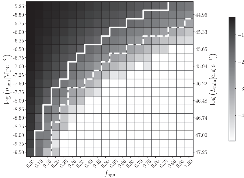
Figure 3. Significance of the rejection of the no-connection hypothesis as a function of the AGN number density ( n_{\text{agn}} ) and the fraction of GW events originated in an AGN ( f_{\text{agn}} ). The p -values (and hence the significance) here represented refer to the detections of 13 events associated with z \leq 0.2 . On the right of the dashed (solid) white line there is the region of the 2D parameter space in which the no-connection hypothesis can be rejected with a 3\sigma ( 2\sigma ) significance. The p -values here represented are obtained from the comparison of the median of the \lambda_s distribution with respect to the \lambda_b distribution. Every value of \lambda_s has been calculated using equation (2) in a simulation in which a fraction f_{\text{agn}} of GWs come from an AGN. On the other hand, every value of \lambda_b comes from a simulation in which no GW event is originated in an AGN. On the right-hand axis, we report the logarithm of the minimum bolometric luminosity L_{\text{min}}[\text{erg s}^{-1}] that has to be considered in the integration of the AGN LUMINOSITY FUNCTION at z = 0.1 (Hopkins et al. 2007) to obtain the value of \log(n_{\text{agn}}[\text{Mpc}^{-3}]) indicated on the left-hand side of the grid.
