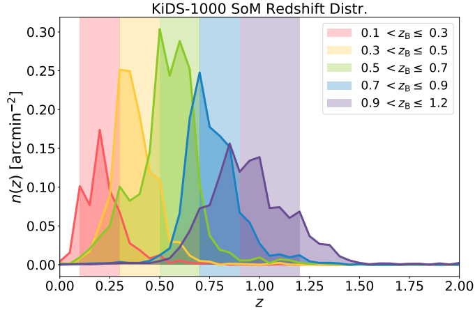
Fig. 1. KiDS-1000 redshift distribution for the five tomographic bins used. Solid lines show the redshift distributions obtained via the SOM technique (Hildebrandt et al. 2021). The shaded bands show the corresponding ranges of photometric redshift point estimates, z_B .
