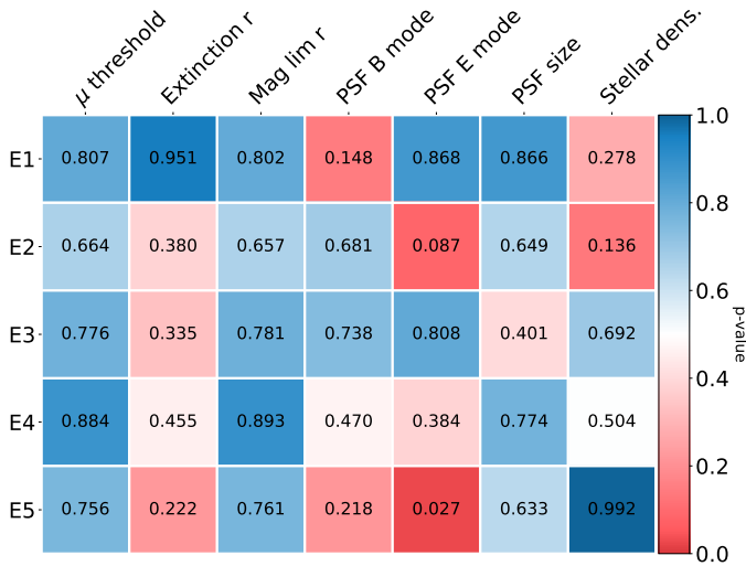
Fig. 6. P-values for the cross-correlations between the data’s tomographic pseudo E-modes and different systematics for a null detection ( p \leq 0.05 would indicate a detection). Here we show the systematics motivated in Sect. 4: object detection threshold ( \mu -threshold), extinction for the r -band, magnitude limit for the r -band, PSF ellipticity components in harmonic space (E/B-mode), the PSF size, and stellar overdensity from Gaia DR2 (Gaia Collaboration et al. 2018). The highest correlation occurs for the PSF E-mode in the fifth tomographic bin, this is shown in Fig. 7 to be subdominant to the cosmological signal given the estimated statistical error in this particular tomographic bin.
