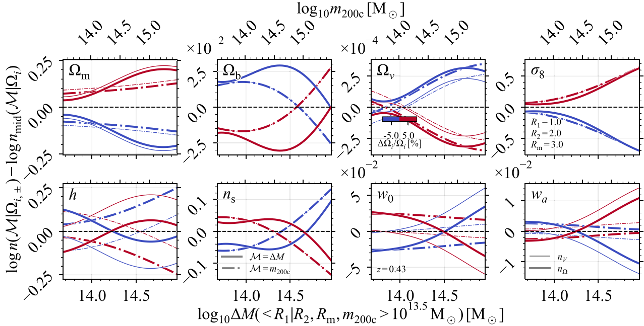
Figure 14. Comparison between the cosmology sensitivity of the 3D halo mass function (dash-dotted lines) and the aperture mass function (solid lines) with ( n_\Omega , thick lines) and without ( n_v , thin lines) including the cosmology dependence of the survey solid angle and redshift interval at z = 0.43 . The cosmological parameter being varied by \pm 5 per cent (coloured lines) with respect to the fiducial Planck Collaboration et al. (2020) cosmology is indicated in the top-left corner of each panel. We assume w_a = \pm 0.05 since the fiducial value is 0. The aperture mass function is plotted for the median aperture mass at m_{200c} for all the simulations in the hypercube, and for apertures (R_1, R_2, R_m) = (1, 2, 3) cMpc. All haloes have m_{200c} > 10^{13.5} M_\odot . The probed comoving volume for a fixed observed area is mainly sensitive to h , \Omega_m , w_0 , and w_a . Compared to the 3D halo mass function, the aperture mass function is more sensitive to the changes in \Omega_m and w_a , similarly sensitive to \sigma_8 and w_0 , and less sensitive to h .
