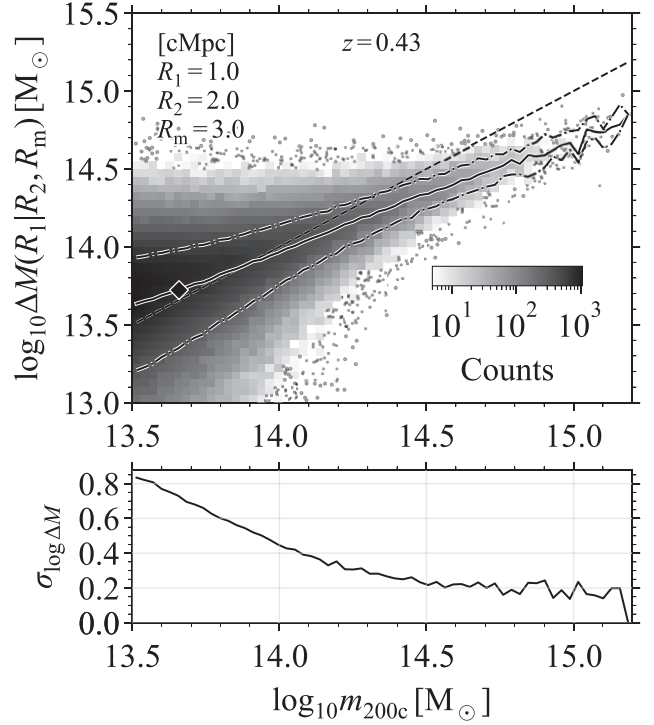
Figure 4. Top panel: The distribution of aperture masses, \Delta M(< R_1 = 1.0 \text{ cMpc} | R_2 = 2.0 \text{ cMpc}, R_m = 3.0 \text{ cMpc}) , as a function of the 3D spherical overdensity mass m_{200c} for simulation M011 at z = 0.43 . The dashed line indicates the one-to-one relation, the solid line indicates the median relation, and the dash-dotted lines indicate the 16–84th percentile scatter. The diamond indicates the 3D halo mass for which r_{200c} = R_1 . The large scatter in \Delta M at fixed m_{200c} is caused by the large variation in the matter distribution along the line-of-sight. Bottom panel: The logarithmic scatter in the aperture mass distribution at fixed m_{200c} , calculated as half the difference between the 84th and the 16th percentiles. The scatter decreases from \sigma_{\log \Delta M} \approx 0.45 at m_{200c} = 10^{14} M_{\odot} to \lesssim 0.2 for m_{200c} > 10^{14.5} M_{\odot} .
