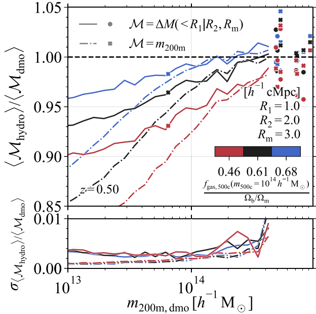
Figure 6. Top panel: The dependence of the suppression in the aperture mass, \Delta \mathcal{M}_{\text{hydro}}(< 1h^{-1} \text{ cMpc} | R_2, R_m) (solid lines), and the 3D halo mass, m_{200\text{m}} (dash-dotted lines) on the halo gas fraction, f_{500\text{c,gas}}(m_{500\text{c}} = 10^{14} h^{-1} M_{\odot}) , relative to the cosmic baryon fraction, \Omega_b/\Omega_m , stacked in bins of the 3D dark matter-only halo mass. All background correction annuli span the region between R_2 = 2 h^{-1} \text{ cMpc} and R_m = 3 h^{-1} \text{ cMpc} . Red (blue) lines show higher (lower) AGN heating temperatures in the simulation, resulting in lower (higher) gas fractions. Crosses indicate the halo mass for which r_{200\text{m,dmo}} = R_1 . Bins with fewer than 5 haloes show the individual suppression ratios. The mass suppression increases with increasing feedback strength and decreasing cluster gas fractions. Aperture masses are consistently suppressed less than the 3D halo mass for m_{200\text{m,dmo}} \lesssim 10^{14} h^{-1} M_{\odot} . Bottom panel: The 1\sigma bootstrapped uncertainty in the mass suppression of hydrodynamical haloes compared to their matched DMO counterparts for the different mass measurements. The uncertainty in the mass suppression only changes slightly for the most massive haloes when changing the simulated AGN feedback.
