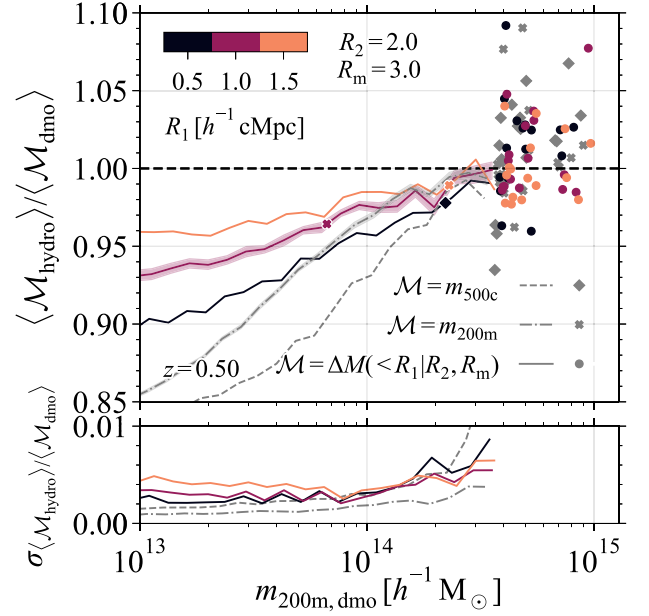
Figure 2. Top panel: The mean aperture mass of haloes in the reference hydrodynamical simulation relative to the mean mass of the matched dark matter-only simulation counterparts at z = 0.5 , stacked in bins of the 3D dark matter-only halo mass. Different coloured lines show different aperture sizes R_1 = [0.5, 1, 1.5] h^{-1} \text{cMpc} , with the background contribution calculated between R_2 = 2 h^{-1} \text{cMpc} and R_m = 3 h^{-1} \text{cMpc} , representative for weak lensing observations. Dash-dotted (dashed) grey lines show the change in the 3D halo mass \langle m_{200\text{m}, \text{hydro}} \rangle / \langle m_{200\text{m}, \text{dmo}} \rangle ( \langle m_{500\text{c}, \text{hydro}} \rangle / \langle m_{500\text{c}, \text{dmo}} \rangle ). Shaded regions show the bootstrapped error on the ratio of the mean masses for m_{200\text{m}} and \Delta\mathcal{M}(< 1 h^{-1} \text{cMpc} | R_2, R_m) . For bins with fewer than 10 haloes, individual measurements are shown with coloured points for the aperture mass, and grey crosses (diamonds) for the 3D halo mass, m_{200\text{m}} ( m_{500\text{c}} ). Coloured crosses (diamonds) show the 3D halo mass for which r_{200\text{m}, \text{dmo}} = R_1 ( r_{500\text{c}, \text{dmo}} = R_1 ). For m_{200\text{m}, \text{dmo}} \gtrsim 10^{14} h^{-1} M_{\odot} , the mass change is < 5 per cent for all mass measures. For halo masses \lesssim 10^{14} h^{-1} M_{\odot} , the aperture mass is consistently less biased than the 3D halo mass. Bottom panel: The 1\sigma bootstrapped uncertainty in the mean mass change is < 1 per cent for all mass measurements. For high-mass haloes, the decrease in the number of haloes causes the larger uncertainty.
