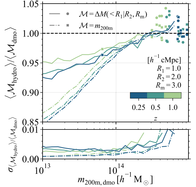
Figure 5. Top panel: The redshift dependence of the change in the aperture mass, \Delta \mathcal{M}_{\text{hydro}}(< 1 h^{-1} \text{cMpc} | R_2, R_m) (solid lines), and the 3D halo mass, m_{200\text{m}} (dash-dotted lines), stacked in bins of the 3D dark matter-only halo mass. All background correction annuli span the region between R_2 = 2 h^{-1} \text{cMpc} and R_m = 3 h^{-1} \text{cMpc} . Coloured lines show the different redshifts and crosses the halo mass for which r_{200\text{m,dmo}} = R_1 . Bins with fewer than 5 haloes show the individual results. The mass reduction decreases with increasing redshift at fixed 3D halo mass. At all redshifts, the aperture mass changes less than the 3D halo mass for m_{200\text{m,dmo}} \lesssim 10^{14} h^{-1} M_{\odot} . Bottom panel: The 1\sigma bootstrapped uncertainty in the mass change of hydrodynamical haloes compared to their matched DMO counterparts for the different mass measurements. The uncertainty in the mass reduction only increases for the rarest, high-mass haloes at higher redshift.
