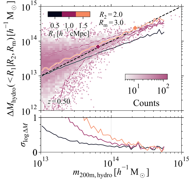
Figure 1. Top panel: The distribution of aperture masses within 1 h^{-1} \text{ cMpc} , \Delta M_{\text{hydro}}(< 1 h^{-1} \text{ cMpc} | R_2 = 2 h^{-1} \text{ cMpc}, R_m = 3 h^{-1} \text{ cMpc}) , as a function of the 3D halo mass, m_{200\text{m,hydro}} , at z = 0.5 . The median relations for different aperture sizes are shown as coloured lines, with the dash-dotted lines indicating the 16th to 84th percentile scatter for R_1 = 1 h^{-1} \text{ cMpc} . The one-to-one relation is indicated by the black, dashed line. The coloured diamonds indicate the halo mass where r_{200\text{m}} = R_1 . There is a large scatter in aperture mass at fixed, low m_{200\text{m,hydro}} due to the variation in the structure along the line of sight to different haloes. The aperture mass tends to be slightly higher (lower) than the 3D halo mass when R_1 > (<) r_{200\text{m,hydro}} . Bottom panel: The logarithmic scatter in the aperture mass at fixed m_{200\text{m,hydro}} , measured as half the difference between the 84th and 16th percentiles. The scatter increases for lower 3D halo masses since matter outside the halo dominates the aperture mass. For m_{200\text{m,hydro}} \lesssim 10^{13.5} h^{-1} M_\odot , the scatter increases significantly since > 5 per cent of the haloes is surrounded by more massive structures resulting in negative aperture masses.
