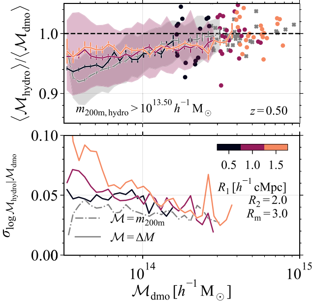
Figure 4. Top panel: The mean bias for the aperture mass (solid lines) and the 3D halo mass (dash-dotted lines) as a function of the corresponding mass of the matching dark matter-only halo at z = 0.5 for all haloes with m_{200\text{m,hydro}} > 10^{13.5} h^{-1} M_{\odot} . Shaded regions show the 1\sigma scatter for R_1 = 1 h^{-1} \text{cMpc} and m_{200\text{m}} . Error bars show the bootstrapped uncertainty on the mean mass bias. Coloured lines show the different aperture sizes R_1 = [0.5, 1, 1.5] h^{-1} \text{cMpc} , with the background contribution calculated within R_2 = 2 h^{-1} \text{cMpc} and R_m = 3 h^{-1} \text{cMpc} . Bins with fewer than 10 haloes show the individual results. Results for aperture and 3D mass measurements are not directly comparable since a fixed \mathcal{M}_{\text{dmo}} corresponds to different haloes. Bottom panel: The 1\sigma scatter in \mathcal{M}_{\text{hydro}} at fixed \mathcal{M}_{\text{dmo}} at z = 0.5 . For all mass measures, the scatter is smaller than \approx 5 per cent for \mathcal{M}_{\text{dmo}} \gtrsim 10^{14} h^{-1} M_{\odot} . For lower masses, the aperture mass scatter increases more than the 3D halo mass scatter due to the contribution of matter outside haloes.
