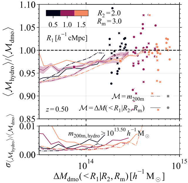
Figure 3. Top panel: The mean aperture mass of haloes, measured within different apertures (solid, coloured lines), in the reference hydrodynamical simulation relative to their matched counterparts from the dark matter-only simulation at z = 0.5 , stacked in bins of the dark matter-only aperture mass for all haloes with m_{200\text{m,hydro}} > 10^{13.5} h^{-1} M_{\odot} . The background contribution to the aperture mass is calculated within R_2 = 2 h^{-1} \text{cMpc} and R_m = 3 h^{-1} \text{cMpc} . Coloured, dash-dotted lines show the 3D halo mass ratio, \langle m_{200\text{m,hydro}} \rangle / \langle m_{200\text{m,dmo}} \rangle , within the different aperture mass bins. Coloured crosses indicate the mean aperture mass for haloes with r_{200\text{m,dmo}} = R_1 . Shaded regions show the bootstrapped error on the ratio of the mean masses for m_{200\text{m}} and \Delta M for R_1 = 1 h^{-1} \text{cMpc} . For bins with fewer than 10 haloes, individual measurements are shown with points and crosses for the aperture mass and the 3D halo mass, respectively. Aperture masses change less than (similarly to) 3D halo masses for haloes with r_{200\text{m,dmo}} \lesssim (\gtrsim) R_1 . Bottom panel: The 1\sigma bootstrapped uncertainty in the mass change for the different mass measures. The uncertainty increases for both low aperture masses with R_1 \gg r_{200\text{m,dmo}} , dominated by matter outside the halo, and high aperture masses due to their lower numbers in BAHAMAS.
