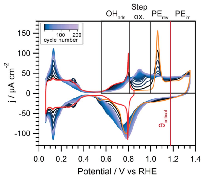
Figure 1. Oxidation-Reduction Cycles on Pt(111). The CV to only 0.85 V and the first ORC are shown in red and in orange, respectively, while the remaining ORCs are indicated according to the color scale. The OH adsorption, step oxidation, PE rev , and PE irr regions are indicated, as well as the voltage at the critical coverage. The scan rate is 50 mV s -1 .
