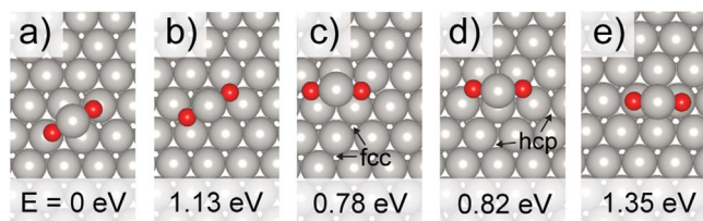
Figure 5. Potential Energy Landscape of a \text{PtO}_2 -adatom ( \text{PE}_{\text{irr}} -adatom) on \text{Pt}(111) : (a) bridge1, (b) atop, (c) fcc, (d) hcp, (e) bridge2. The lowest energy state, the energy of a \text{PtO}_2 -adatom at bridge1, is used as reference. The diffusion barrier of a \text{PtO}_2 -adatom must be at least 0.78 eV.
