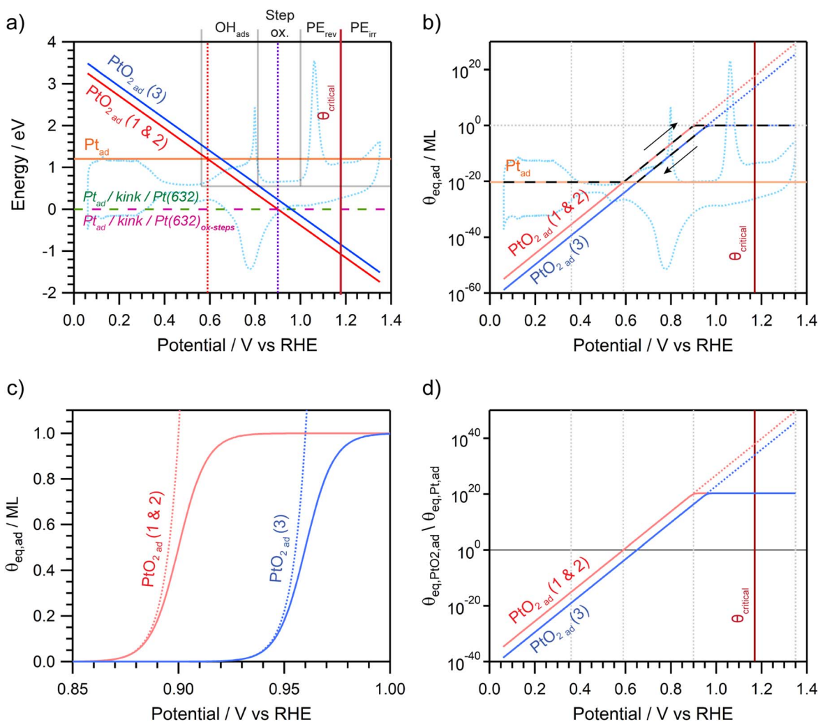
Figure 3. Formation Energies and Concentrations of Adatoms. (a) The formation energies of a Pt-adatom and a \text{PtO}_2 -adatom on Pt(111), and a \text{PtO}_2 -adatom on a Pt(111) with 4/25 ML \text{O}_{ads} , are shown in orange, red, and blue, respectively. They are referenced with respect to the binding energy of an additional Pt atom attached directly to a kink site on Pt(632), which can be unoxidized (green dashed line) or oxidized (pink dashed line). The numbers in brackets indicate the reactions considered, explained in the main text. The dotted red and purple lines indicate the Pt-adatom oxidation potential and the potential at which E_{\text{PtO}_{2,ad}} (1&2) becomes zero, respectively. The first ORC is shown in dotted light blue and the different regions are indicated. (b) Equilibrium Pt- and \text{PtO}_2 -adatom concentrations calculated from (a). The dotted red and blue lines result from the Boltzmann equation with the approximation which match, respectively, the solid red and blue lines (considering the complete entropy term without approximation) at potentials <0.85 V. The dashed black line and the arrows indicate the path followed upon one ORC, while the vertical lines indicate the potentials that are provided also in Table I. (c) Zoomed-in graph of the region between 0.85 V and 1.00 V in (b). (d) Concentration ratios between \text{PtO}_2 - and Pt-adatoms.
