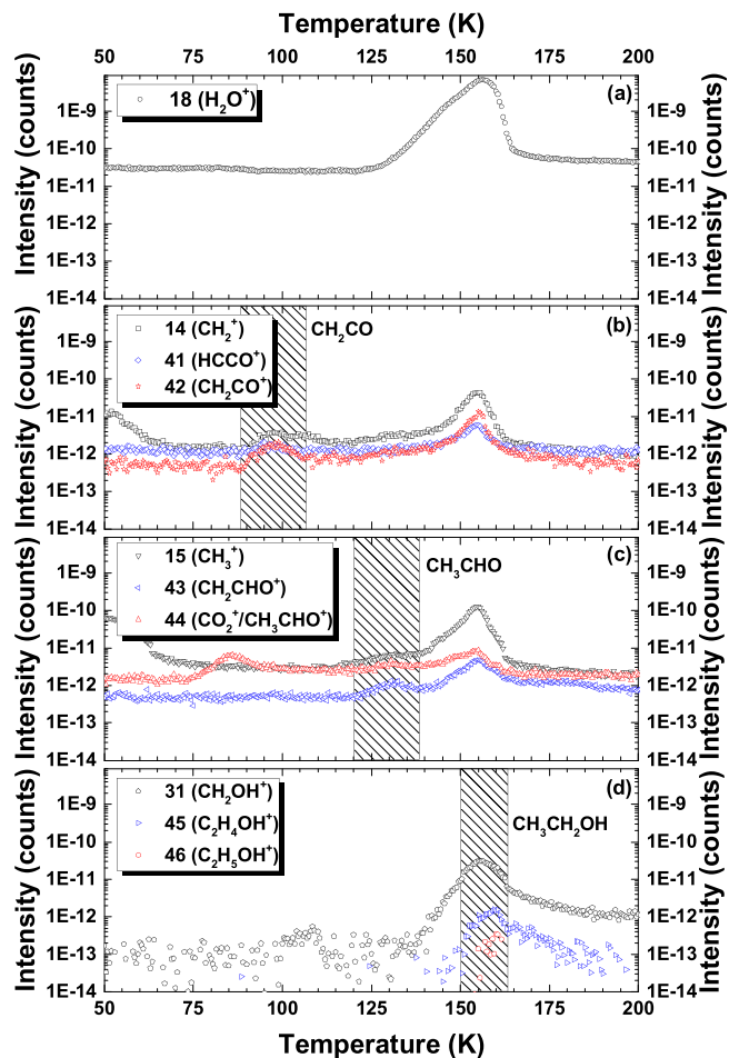
Figure 2. Four different mass settings for a TPD-QMS experiment performed after the simultaneous codeposition of \text{H}_2\text{O} molecules with C atoms, CO molecules, and H atoms on a 10 K substrate for 1920 s. The \text{H}_2\text{O}:\text{C}:\text{CO}:\text{H} ratio is estimated to be 16:1:1.5:4 with a C-atom flux equal to 5 \times 10^{11} \text{ cm}^{-2} . For clarity, the m/z plots are presented in distinct groups with characteristic m/z signals of (a) \text{H}_2\text{O}^+ , (b) \text{CH}_2\text{CO}^+ (ketene), (c) \text{CH}_3\text{CHO}^+ (acetaldehyde), and (d) \text{CH}_3\text{CH}_2\text{OH}^+ (ethanol), respectively. The patterned boxes indicate the gas-phase detections of the various species at their characteristic desorption temperatures. The m/z = 18 ( \text{H}_2\text{O}^+ ) plot is shown to demonstrate that a vast fraction of the species formed, is expected to be entrapped in \text{H}_2\text{O} ice and released into the gas phase upon the sublimation of \text{H}_2\text{O} ice. Spectra are presented without an offset for direct comparison.
