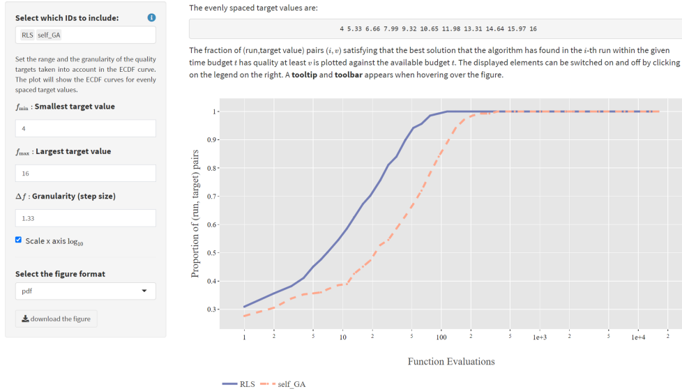
Fig. 8. Screenshot of aggregated ECDF curve over multiple targets.
