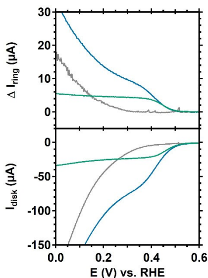
Figure 2. Linear sweep voltammograms with a rotating ring disk electrode setup of 0.15 mm \text{Cu}_2(\text{btmipa}) under argon (green) and \text{O}_2 atmosphere (blue). The cyclic voltammogram of the GC disk (bottom panel) and the current response of the Pt ring (top panel) are shown. The grey line represents the GC disk in catalyst-free, \text{O}_2 purged electrolyte. The voltammograms were recorded at 50 mV/s in a 0.1 M phosphate buffer of pH 7. A rotation rate of 1600 rpm and a Pt ring potential of 1.2 V were applied.
