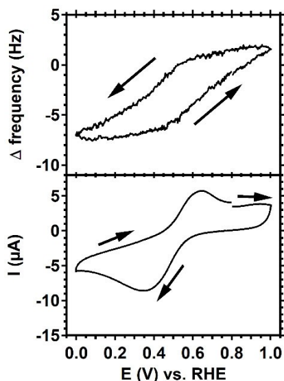
Figure 1. Electrochemical quartz crystal microbalance measurement with a gold work electrode of 0.15 mm \text{Cu}_2(\text{btmipa}) in 0.1 M phosphate buffer of pH 7. The bottom panel shows the second scan of a CV at 50 mV/s scan rate under argon atmosphere. The top panel shows the relative frequency of the quartz crystal and its response with respect to the applied potential.
