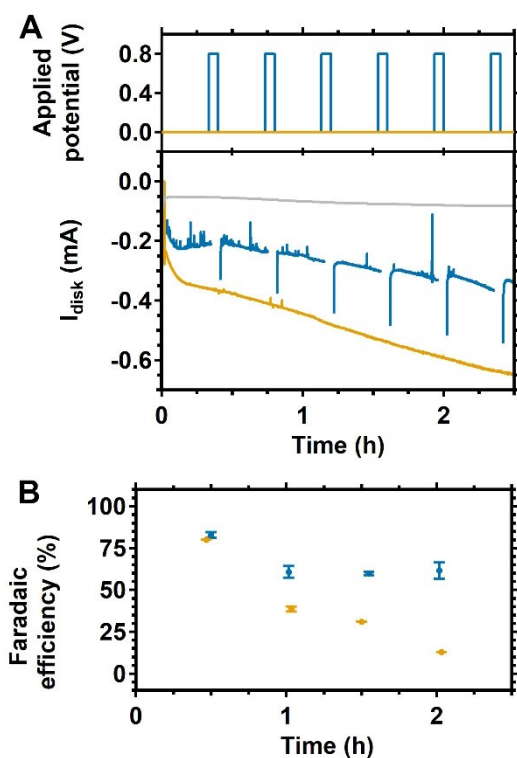
Figure 3. Rotating disk chronoamperometry of a GC disk at 0.0 V in a \text{O}_2 saturated \text{Cu}_2(\text{btmbpa}) solution in a continuous measurement (orange) or a 20 minute interval measurement (blue). For the latter, a 0.8 V potential was applied for 4 minutes to re-oxidize adsorbed \text{Cu}^0 deposition every 20 minutes according to the sequence shown in panel (A). The Faradaic efficiency for \text{H}_2\text{O}_2 is given in (B). The black dots represent the Faradaic efficiency of the time window since the last \text{H}_2\text{O}_2 measurement. The disk was rotated at 1600 rpm in a 0.1 M phosphate buffer of pH 7 with 0.15 mM catalyst.
