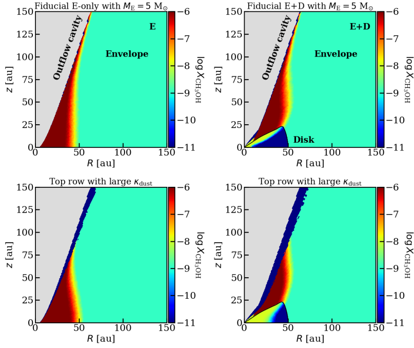
Fig. E.3. Methanol abundance maps for the envelope-only (left) and envelope-plus-disk (right) models when the envelope mass is 5 M_\odot and the other parameters are the same as the fiducial model. The top row shows the models with low mm opacity grains, and the bottom row shows the models with high mm opacity grains. The photodissociation regions for M_E = 5 M_\odot models are very small, and they are similar in models with low and high mm opacity grains, which is different from the fiducial model in Fig. 4.
