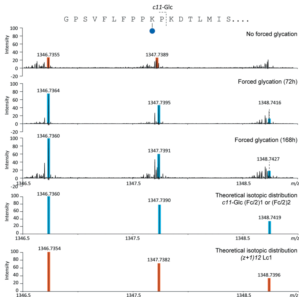
Figure 6. Enlargement of an aFT MALDI-MSD FT-ICR MS spectrum generated from the analysis of non-glycated and glycated IdeS-digested A2V mAb.
