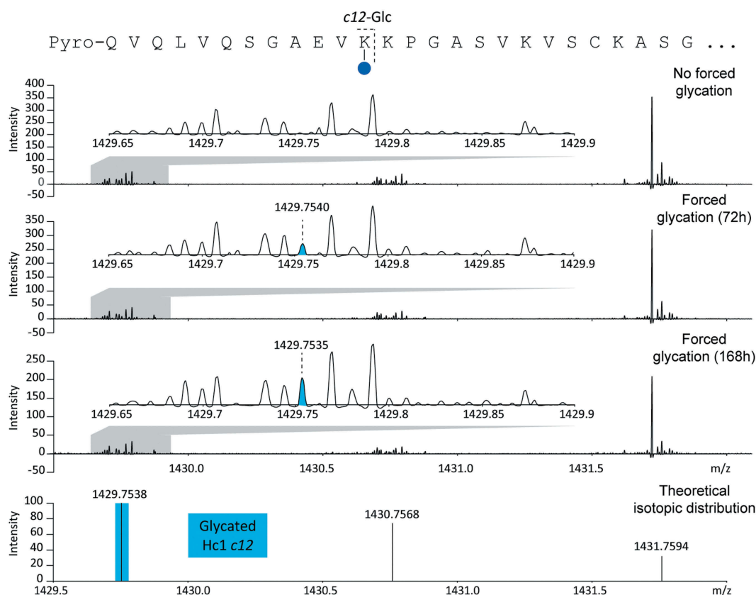
Figure 5. Enlargement of an aFT MALDI-ICR MS spectrum generated from the analysis of non-glycated and glycated intact A2V mAb. Detection of a glycated c12 fragment ion of Hc1 allowed the identification of a glycation site on Lys12.
