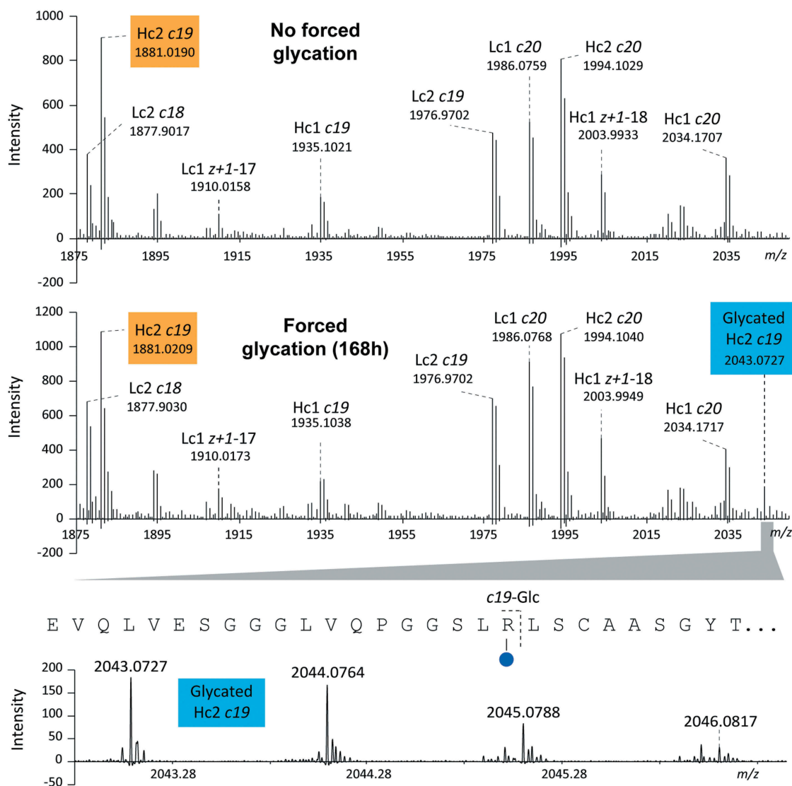
Figure 4. Enlargement of the aFT MALDI-ITD FT-ICR MS spectra obtained from non-glycated (top) and glycated (bottom) intact A2V BsAb. Both non-glycated and glycated c19 fragment ion from Hc2 were detected at m/z 1881.0209 and 2043.0727, respectively, after a 168 h incubation with glucose.
