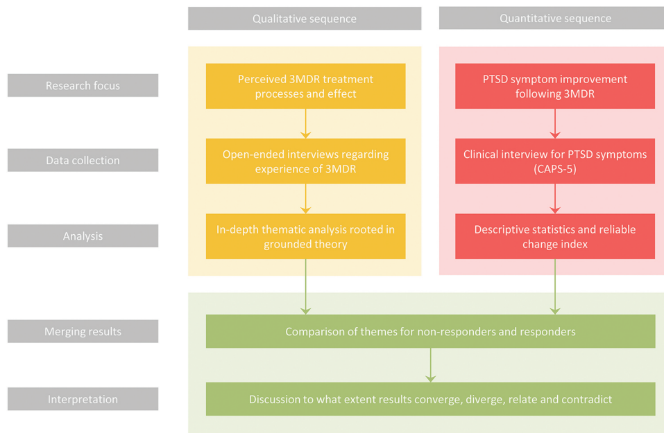
Figure 1. Flow chart of the convergent parallel mixed methods design: two strands of complementary qualitative and quantitative data were collected and analyzed independently and then interpreted together to examine conformity, contradictions and relationships between the two sources of data.
