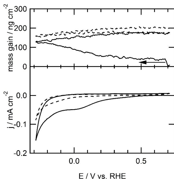
Figure 3. First scan (solid line) and second scan (dotted line) of electrochemical immobilization of 2 at a gold electrode (0.39 cm 2 ) in combination with EQCM of bromobenzene by reduction of a 1 mM 2-N 2 + ion solution generated in situ by addition of 4-bromoaniline and sodium nitrite to form a 1 mM solution of both in 0.5 M HCl electrolyte solution at 100 mV s -1 .
