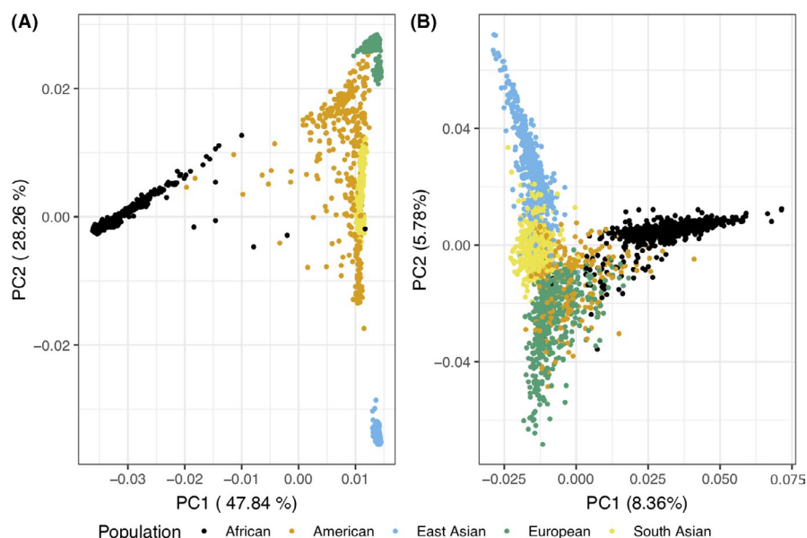
FIGURE 3 A, From 1000 Genomes, first two principal components (PCs) of global genotyping reveals genetic heterogeneity among continental populations. B, From 1000 Genomes, first two PCs of HLA-specific genotyping accounts for a strikingly high proportion of diversity among continental populations
