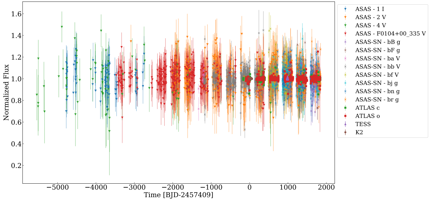
Fig. 4: Time-series photometry of EPIC 2202 from several ground-based surveys as well as the K2 and TESS data. Photometry with a flux value greater than 150% or less than 10% was excluded, along with flux errors error greater than 100%.
