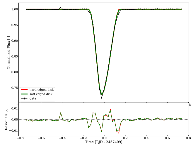
Fig. 7: A comparison of the hard edged model and the soft edged model with residuals.
