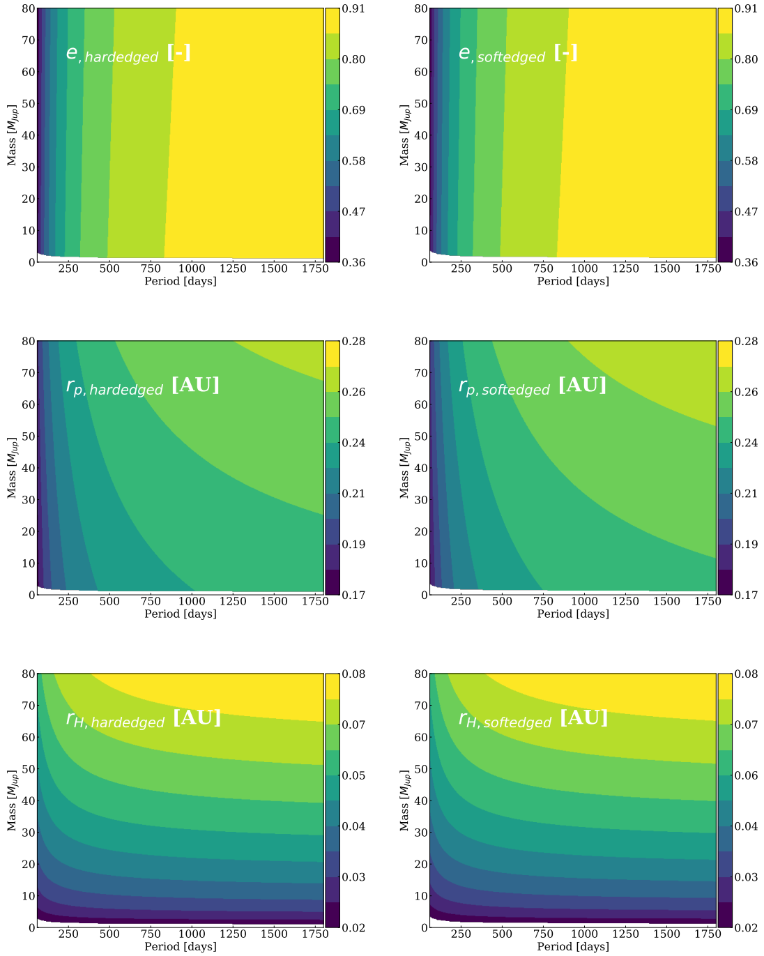
Fig. 9: Parameter space maps for a period between 60 and 1800 days and mass between 0 and 80 M_{\text{Jup}} . The left side is the hard edged disk, the right side is the soft edged disk. The white space at the bottom of the plots is from the constraint R_d < 0.3 r_H .
