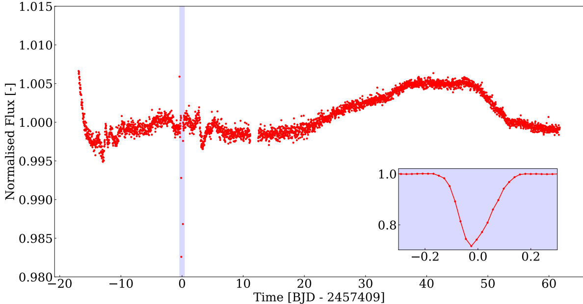
Fig. 1: EVEREST 2.0 light curve of EPIC 2202 with the eclipse centered at BJD 2457409, highlighted in pale blue. Points with non-zero QUALITY values are removed, and the eclipse points have been added back into the light curve (these were incorrectly removed in the pipeline).
