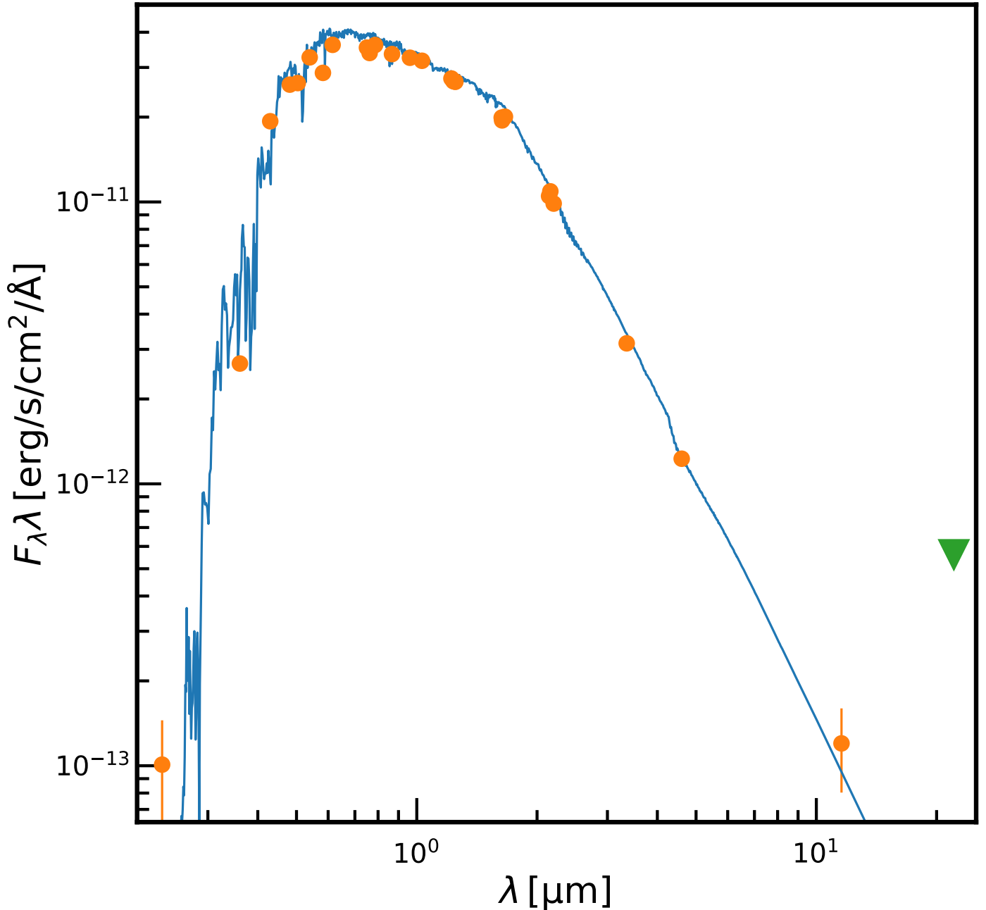
Fig. 3: The spectral energy distribution for EPIC 2202. The blue curve is a Kurucz best fit model. The orange points are the photometry as compiled from SIMBAD. The green triangle is an upper limit measurement from WISE at 22 microns.
