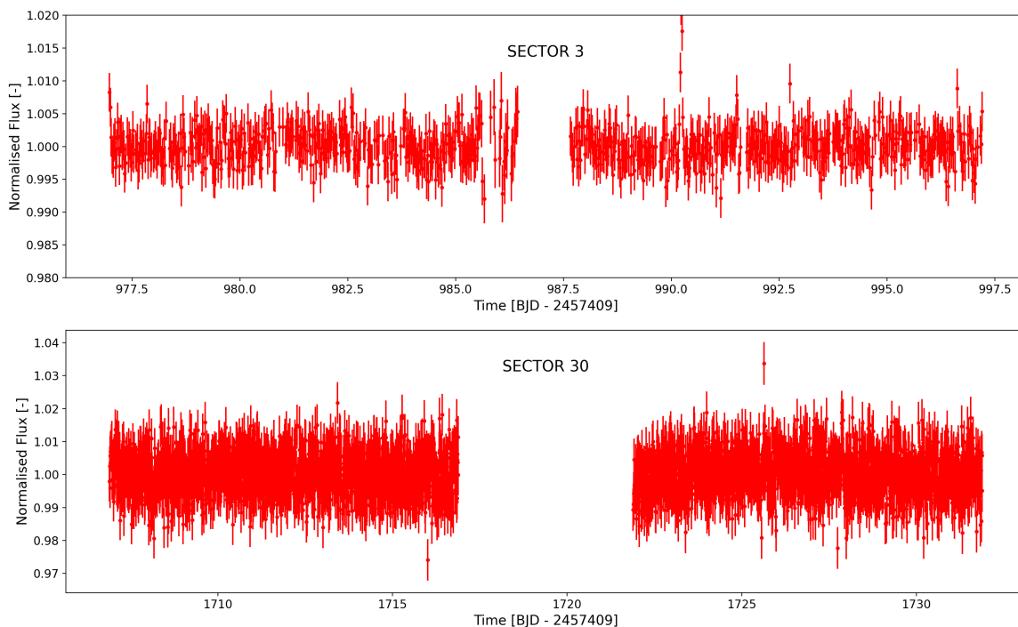
Fig. 2: The eleanor light curve of EPIC 2202. The upper panel shows Sector 3 and the lower panel shows Sector 30. Note that in Sector 30 there was significantly more scattered light, which explains the larger scatter and the larger absence of data between the two orbits.
