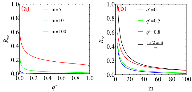
Figure 3. Strong EN, signalled by a positive limiting entropy ratio R_\infty^- > 0 , for weighted matrices under homogeneous one-sided local constraints ( r_i^* = r^* \forall i ) in the dense case with finite m and r^* . (a) R_\infty^- as a function of q^* = \frac{r^*}{m+r^*} for various values of m . Note that R_\infty^- is larger for smaller m and q^* . (b) R_\infty^- as a function of m for various values of q^* . As in the binary case, R_\infty^- decays like \ln(2\pi m)/m as m grows.
