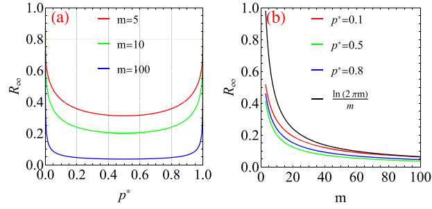
Figure 2. Strong EN, signalled by a positive limiting entropy ratio R_\infty^+ > 0 , for binary matrices under homogeneous one-sided local constraints ( r_i^* = r^* \forall i ) in the dense case with finite m and r^* . (a) R_\infty^+ as a function of p^* = r^*/m for various values of m . Note that R_\infty^+ is larger for smaller m and for values of p^* more distant from the uniform case ( p^* = 1/2 ). (b) R_\infty^+ as a function of m for various values of p^* . Note that, as m grows, R_\infty^+ decays like \ln(2\pi m)/m .
