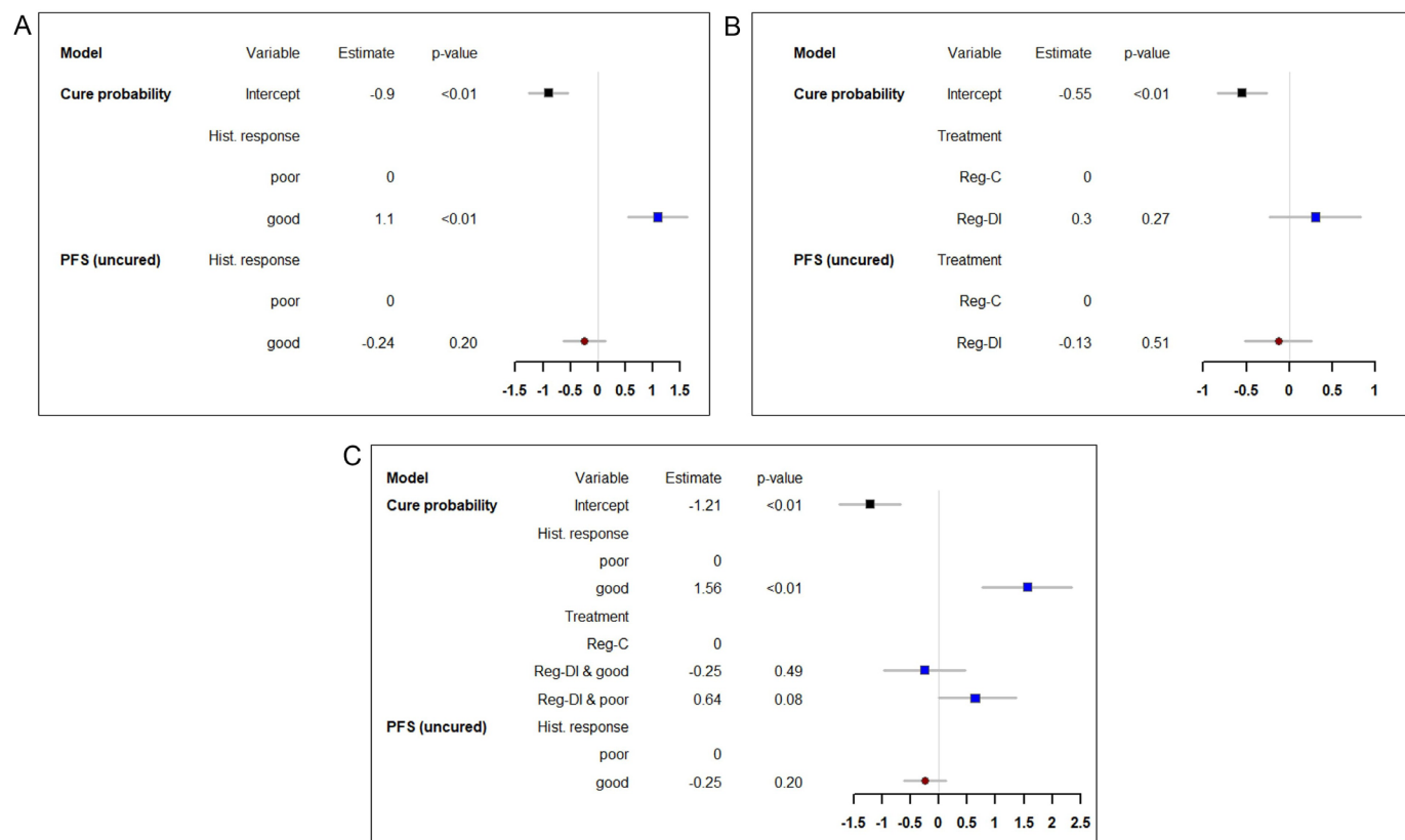
Figure 3 Parameter estimates, 95% CIs and p values for the fitted univariate cure models based on histological response (A), allocated treatment (B) and the multivariate cure model (C). For each univariate or multivariate model, coefficients corresponding to the variables included in the cure probability model and in the PFS model for the uncured, are estimated jointly. Blue squares and red circles represent logORs and logHRs respectively. DI, dose-intensified; PFS, progression-free survival.
