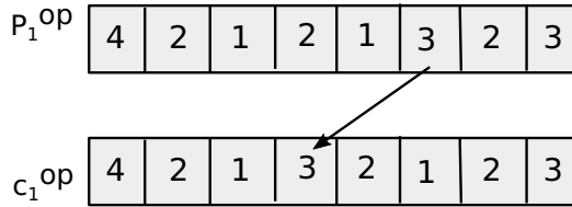
Figure 7.5: Mutation of the operation sequence vector. Adapted from [241].
