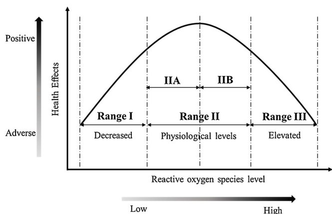
Fig. 1. ROS levels and health effects: a dose-response model.
