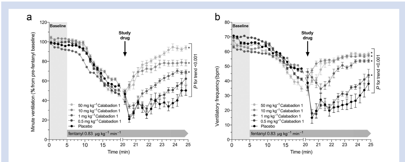
Fig 1. Reversal of fentanyl-induced hypopnea by Calabadiion 1. (a) Minute ventilation and (b) ventilatory frequency were measured after increasing bolus dose of i.v. Calabadiion 1 compared with placebo during a constant-rate fentanyl infusion in orotracheally intubated rats, spontaneously breathing 1.5 vol% isoflurane in air in a randomised crossover model ( n=6 ). Data points represent mean (standard error of the mean) in percent of pre-fentanyl baseline. Across all experiments, minute ventilation and ventilatory frequency significantly decreased after 15 min of fentanyl infusion ( P<0.001 ). Calabadiion 1 dose dependently ( P for trend <0.001 ) enhanced recovery from fentanyl-induced hypopnea at doses greater or equal to 1\text{ mg kg}^{-1} compared with placebo. Asterisks indicate statistical significance compared with placebo ( *P<0.05 ).
