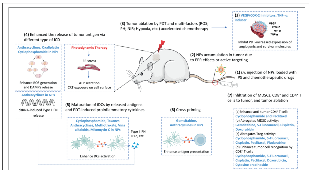
Figure 2. The mechanisms of NP-mediated chemo-photodynamic therapy enhance monotherapy indices and synergistically trigger robust antitumor immune responses for anti-primary and metastatic tumors: (1) intravenous injection of PSs and chemotherapeutic agents loaded with nanoparticles; (2) enhanced NP accumulation in tumor due to the tumor-targeting capability of NPs (EPR effects and targeting motif modification on NP surface); (3) primary tumor ablation by enhanced PDT and chemotherapy. PDT-caused vasculature rupture induced surviving tumor cells to produce more protumor factors in the tumor microenvironment. Antiangiogenic mediators, such as VEGF and COX-2 inhibitors, help PDT to achieve more powerful tumor destruction and a lower recurrence or metastasis rate, by blocking tumor angiogenic activity molecules or their receptors; (4) PDT and chemotherapy (anthracyclines, cyclophosphamide, and oxaliplatin) of the primary tumor to induce higher ICD levels and the release of tumor-associated antigens. Anthracyclines also induce dsRNA release from dead tumor cells, which can activate tumor-specific CD8 + T cells by binding to Toll-like receptor-3 and inducing type I interferon production; (5) DC maturation and antigen presentation are enhanced by PDT-generated antigens, proinflammatory cytokines, and chemotherapeutic agents; (6) cross-priming in tumor lymph node; (7) Chemotherapeutic agents in NPs can improve PDT-induced immune responses by modulating the activity of immune cell subsets and by promoting tumor cell death.
