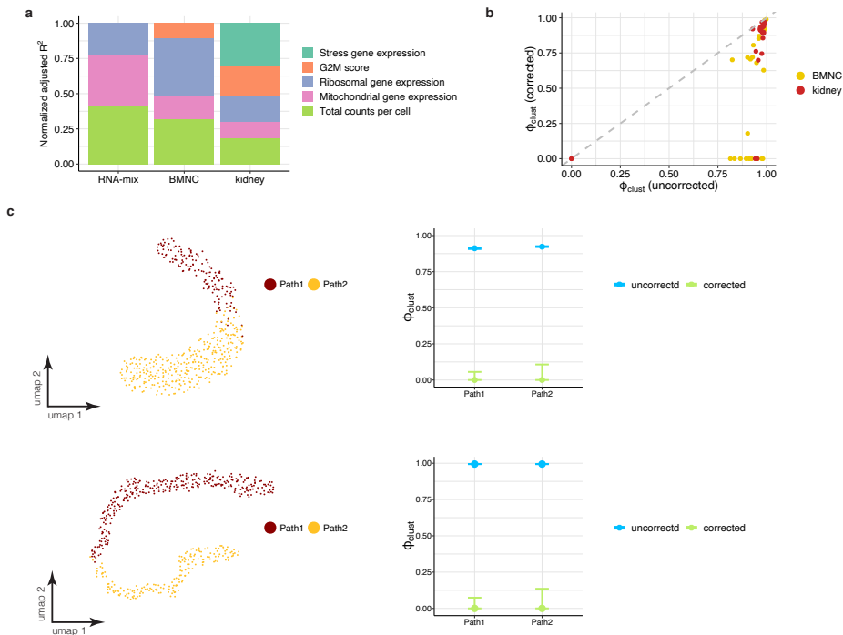
Figure 2.7: Correcting for nuisance parameters and unwanted variability. a Summary of adjusted R^2 for several nuisance parameters in all experimental data sets. b Original (uncorrected) phiclust values vs phiclust corrected for the influence nuisance parameters in the BMNC and fetal kidney data sets. Dashed grey line indicates diagonal. c Two examples of differentiation paths with different numbers of differentially expressed genes. Left: UMAPs of simulated data sets with two differentiation paths. Right: Original (uncorrected) values of phiclust and phiclust values corrected by confounder regression using pseudotime as the only confounder.
