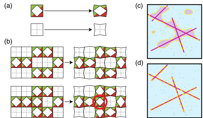
FIG. 1. (a) The building block of [51] can be tiled in two orientations (left) that have a distinct deformation in two dimensions (right). (b) The building blocks of (a) combine into larger designs (structures) that are either C (top) or I (bottom). A change of a single building block can frustrate the deformation (red circle) and change the structure from one that hosts a zero mode (a deformation that costs no energy) ( C ) to one that does not host a zero mode ( I ). A set of rules can be formulated for a unit cell design to have a zero mode [51]. (c) and (d) Conceptual configuration spaces of a discrete combinatorial metamaterial problem. Class C (pink lines) exists in a background of class I (blue), is sensitive to perturbations, and has a complex filamentous structure. Distinguishing between a network with a “coarse” decision boundary (purple dashed line) (c) versus a network with a “fine” decision boundary (d) is not possible with the test set (green dots) due to the undersampled C - I boundary.
