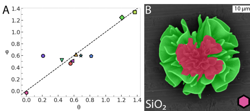
Figure 4. Influence of the silica matrix on shape adaptability during ion exchange. (A) Silica-adjusted volume ratio \varphi (= (\epsilon - \lambda) / (1 - \lambda)) plotted against the formula unit adjusted unit cell volume ratio \theta . Note that compared to Figure 3B, this plot includes an extra datapoint at \theta = 0 for a conversion in which all nanocrystals are removed. (B) Complete removal of nanocrystals from \text{CdCO}_3/\text{SiO}_2 (green) results in a silica structure (red, hexagon symbol in Figure 4A), which albeit shrunk more than five times still exhibits the form and fine details of the original composite, demonstrating shape preservation and the adaptability of the silica matrix.
