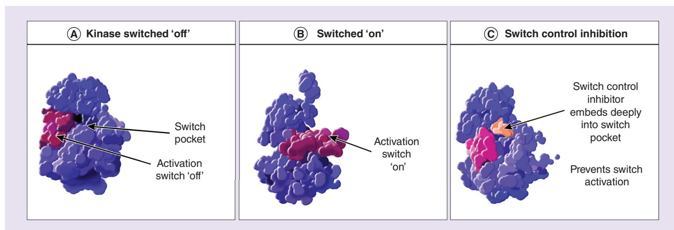
Figure 4. KIT/PDGFRα switch pocket. Kinases have embedded switching mechanisms that conformationally regulate activity. (A) Inactive form of KIT. Note that the activation switch (exon 17, shown in magenta) has not engaged the switch pocket. (B) Active form of KIT. Note that the activation switch has now moved to engage the switch pocket. (C) Ripretinib, a novel tyrosine switch control inhibitor, binds into key regions of the switch pocket, directly inhibiting access by aggressively mutant exon 17 KIT activation loop switches.
